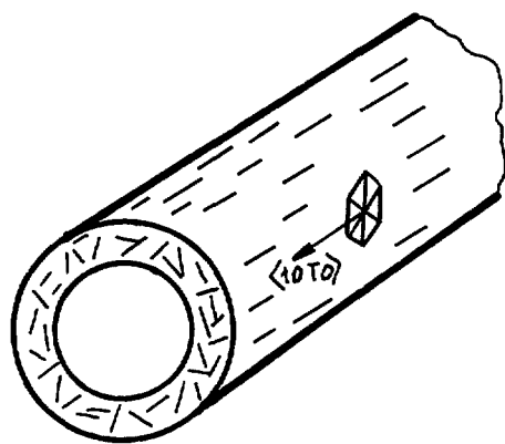
Fig. 12 Basal plane projections in hot extruded beryllium tube
