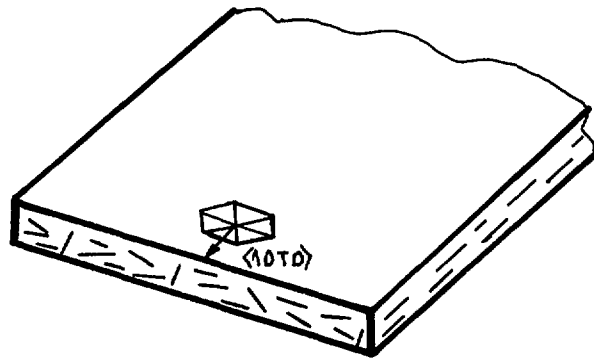
Fig. 8 Basal plane projections in beryllium strip
