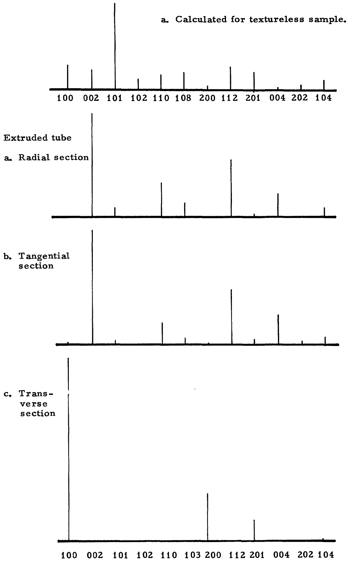
Fig. 11 Extruded tube Relative X-ray intensities for lattice planes parallel to specimen surface
