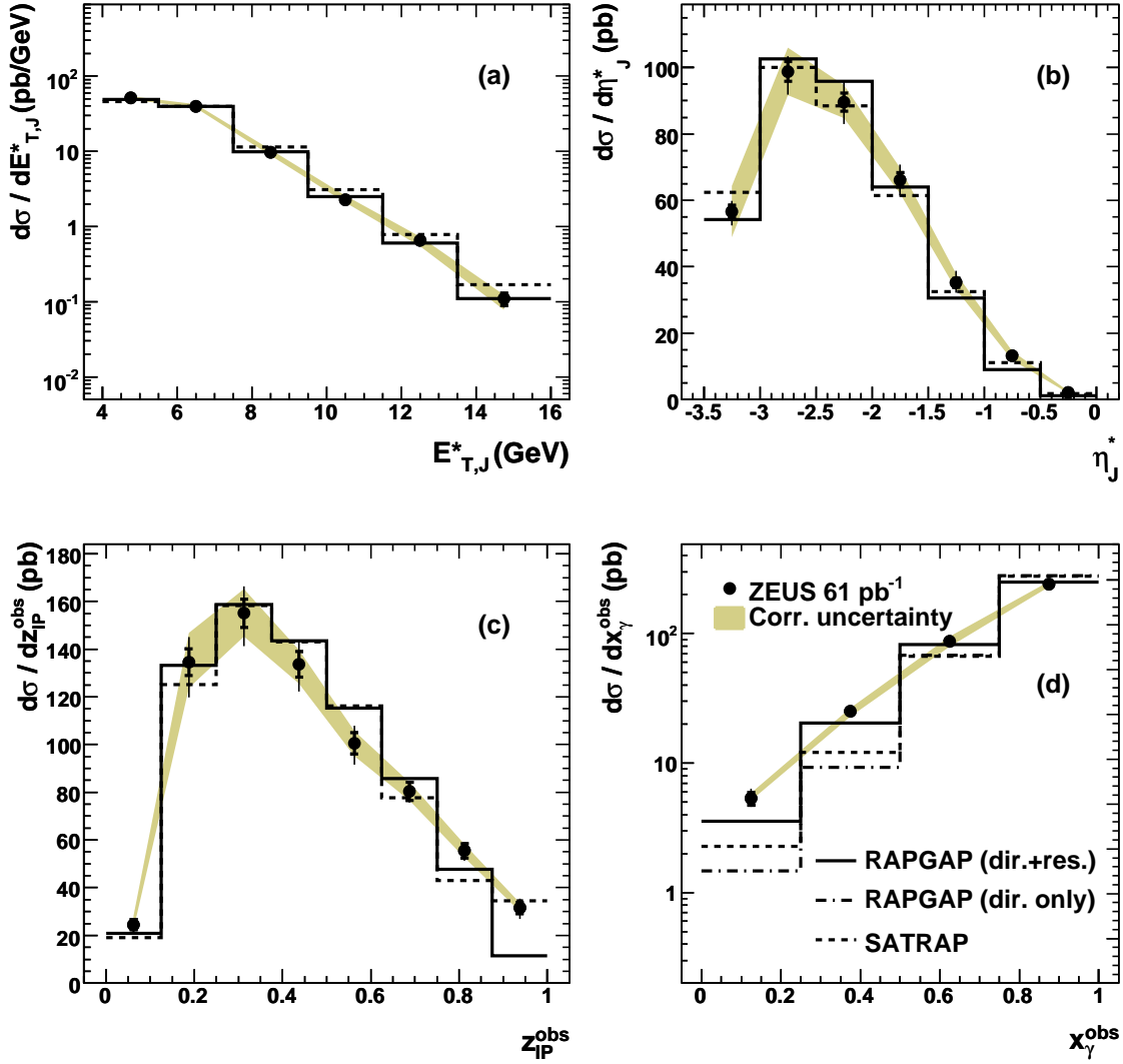
Figure 4: Measured differential cross section as a function of (a) E_{T,J}^* , (b) \eta_J^* , (c) z_{IP}^{\text{obs}} and (d) x_\gamma^{\text{obs}} . The dashed-dotted line represents the area-normalised RAPGAP with only the direct photon contribution. Other details as in the caption of Fig. 3.
