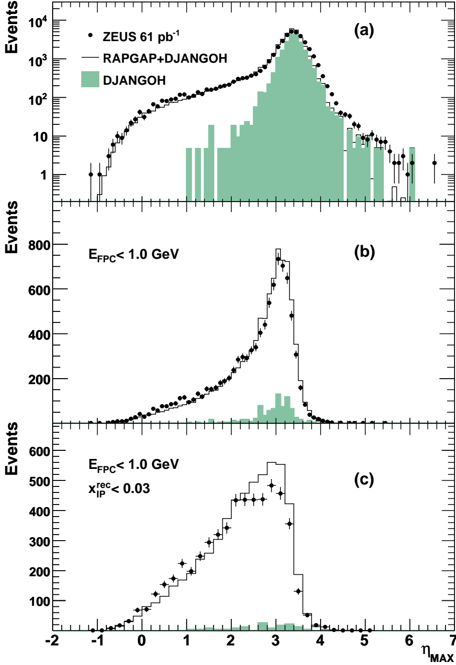
Figure 2: The measured \eta_{\text{MAX}} distribution (dots) (a) before diffractive selection, (b) after the E_{\text{FPC}} < 1.0 \text{ GeV} and (c) after adding the x_{\text{IP}}^{\text{obs}} < 0.03 cut. Also shown are area-normalised MC expectations obtained by fitting the relative amount of RAPGAP and DJANGOH to give the best description of the data before any diffractive selection.
