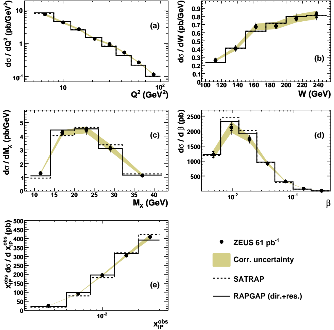
Figure 3: Measured differential cross section (dots) as a function of (a) Q^2 , (b) W , (c) M_X , (d) \beta and (e) x_p^{\text{obs}} . The inner error bars represent the statistical uncertainty and the outer error bars represent the statistical and uncorrelated systematic uncertainties added in quadrature. The shaded band represents the correlated uncertainty. For comparison the area-normalised predictions of the RAPGAP (solid lines) and the SATRAP (dashed lines) MC models are also shown.
