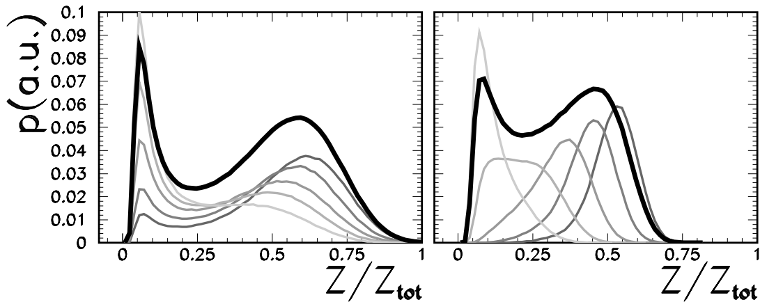
FIG. 5: Distributions of the size of the largest cluster for a system of N=216 particles within the isobar lattice gas model at subcritical pressure. Left: canonical calculations at temperatures T = 3.72, 3.74, 3.76, 3.78, 3.80 MeV close to the transition temperature (thin lines), and their sum (thick line) obtained weighting evenly the different temperatures. Right: microcanonical distributions at energies spanning the coexistence region E/N = 0.75, 1.25, 1.75, 2.25, 2.75 MeV (thin lines), and their sum (thick line) obtained weighting evenly the different energies. The closest neighbors coupling is fixed to \epsilon = 5.5 MeV.
