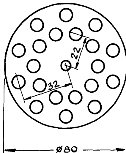
Fig.1. Arrangement for simultaneous irradiation of 60 samples in 3 layers.
