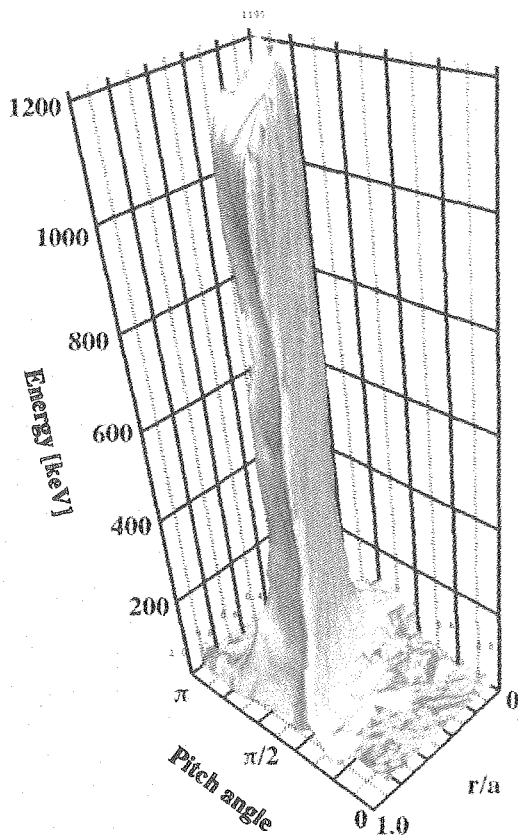
FIG. 2 Steady state distribution of beam ions in the (r/a, E, \text{pitch angle}) space with 2nd harmonics ICRF heating.
