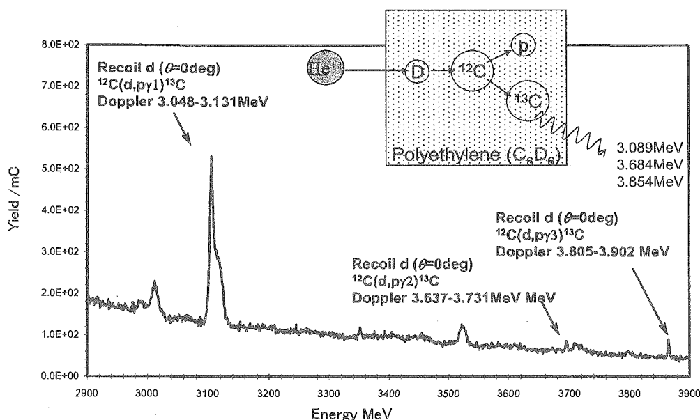
Fig.5 The gamma-peak from sequential ^{12}\text{C}(d,p)^{13}\text{C} reaction induced elastic recoil deuteron.
