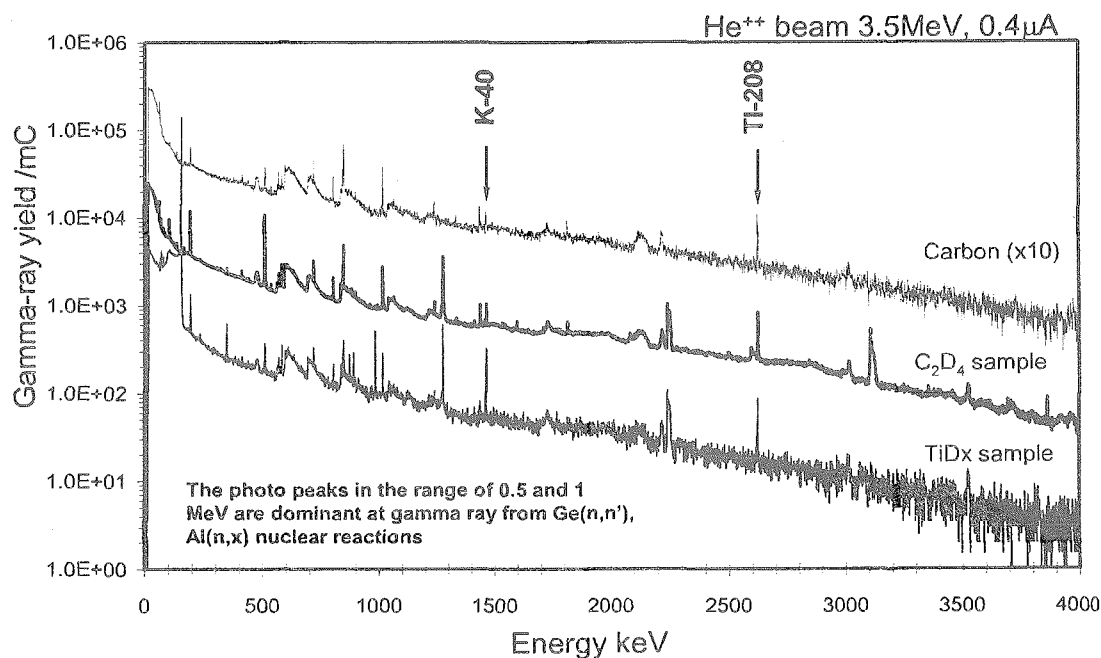
Fig. 3 shows the measured gamma-ray from used C_6D_6 , carbon and TiD_x under 3.5-MeV He^{++} irradiation.
