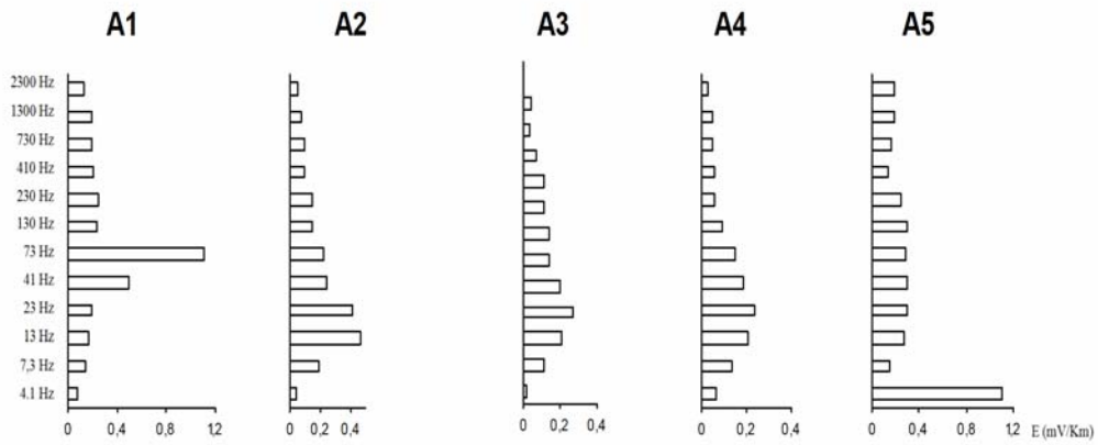
Figure 3b. Propagation of E along profile A telluric line N30°.
