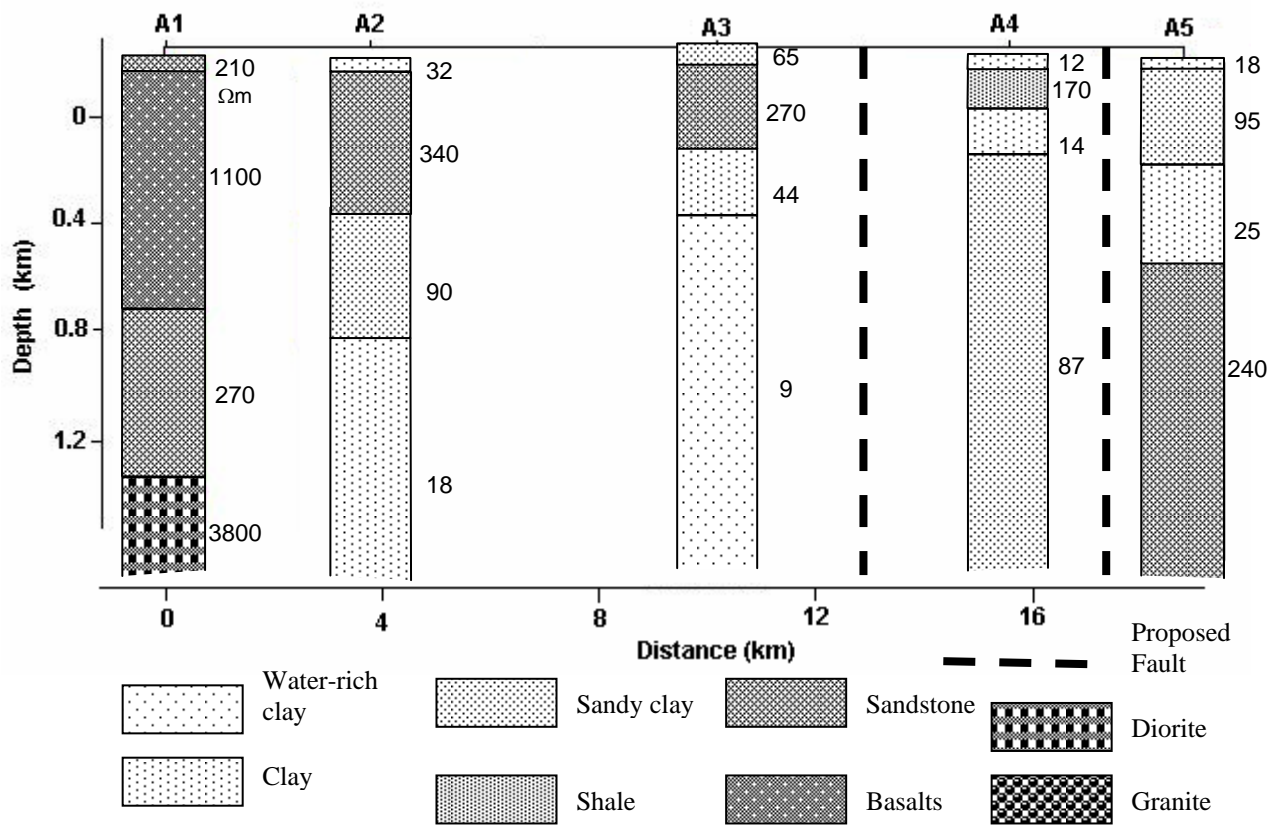
Figure 12. Longitudinal geoelectric section of profile A. Numbers represent resistivities in Ohm-m.
