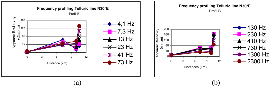
Figure 8. Frequency profiling for profile B in the longitudinal direction.
