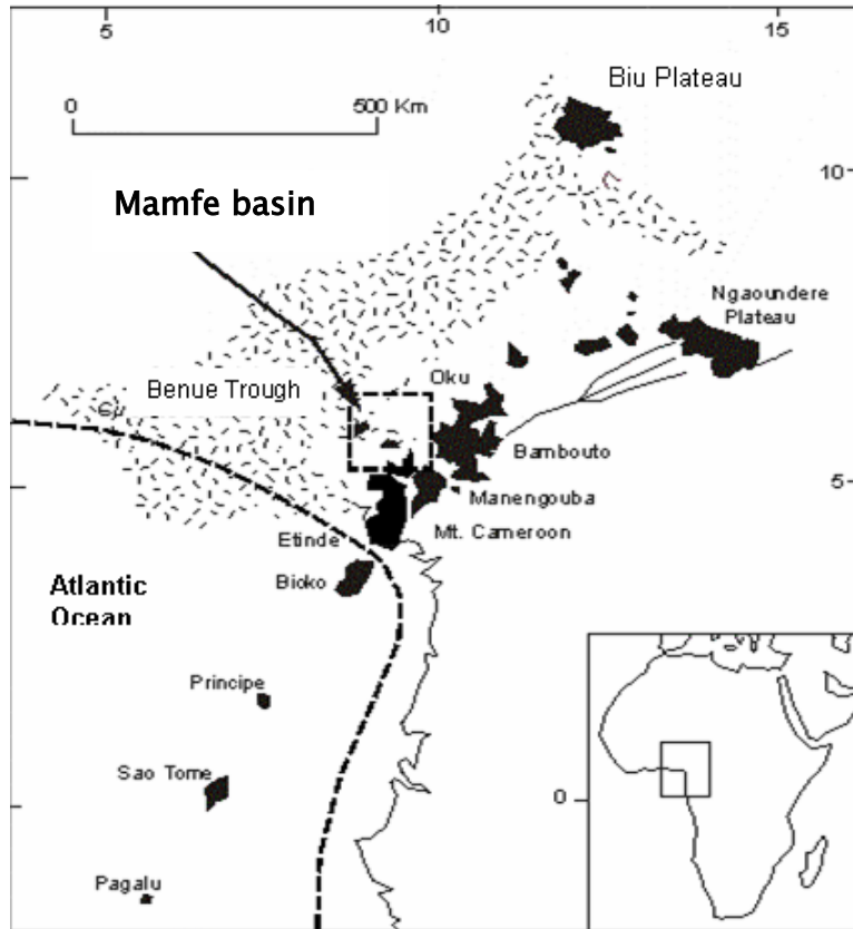
Figure 1. Location of the Mamfe sedimentary basin. The shaded area represents sediments and the volcanics are shown as black spots (after Ngando et al 2004).
