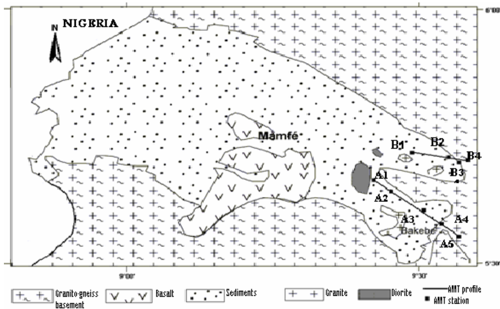
Figure 2. Simplified geologic map of the Mamfe basin showing AMT stations (modified from Dumort 1968).
