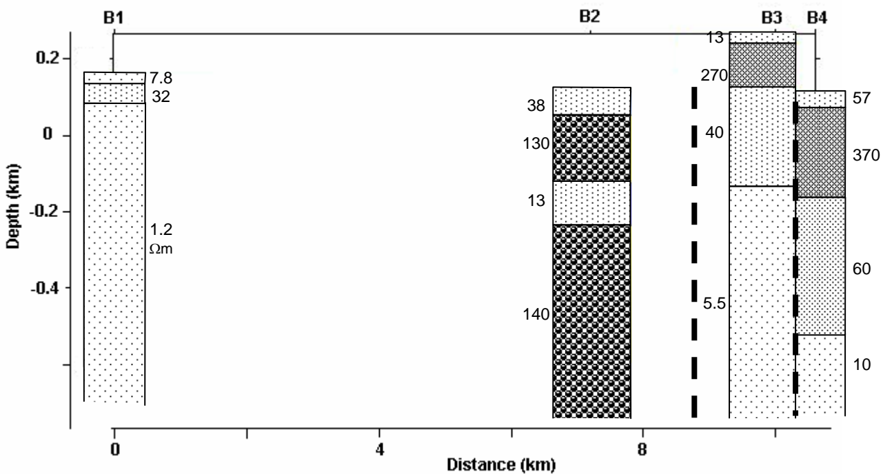
Figure 13. Longitudinal geoelectric section for profile B. (See figure 12 for legend)
