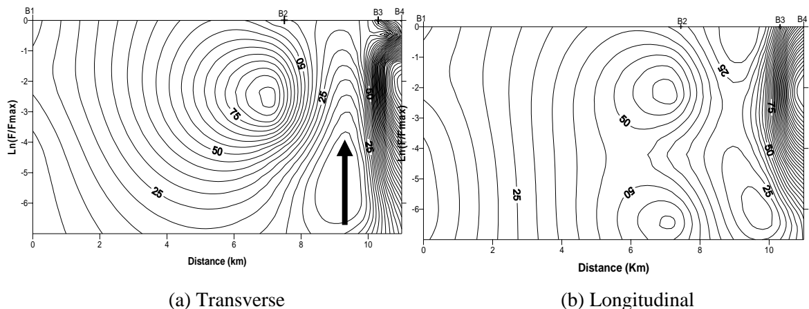
Figure 10. Pseudosection for profile B (arrow shows possible vertical motion of block).
