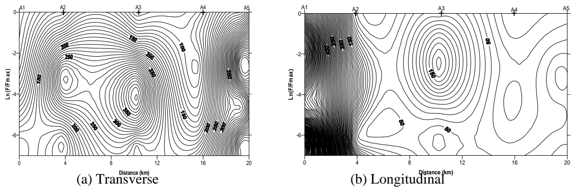
Figure 9. Pseudosection for profile A.
