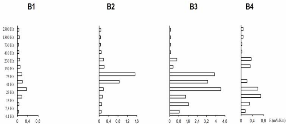
Figure 4a. Propagation of E along profile B telluric line N120°.
