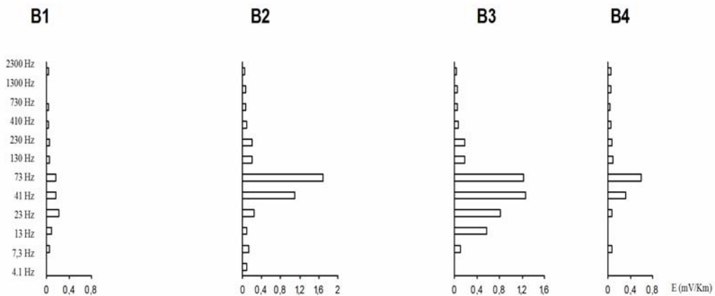
Figure 4b. Propagation of E along profile B telluric line N30°.
