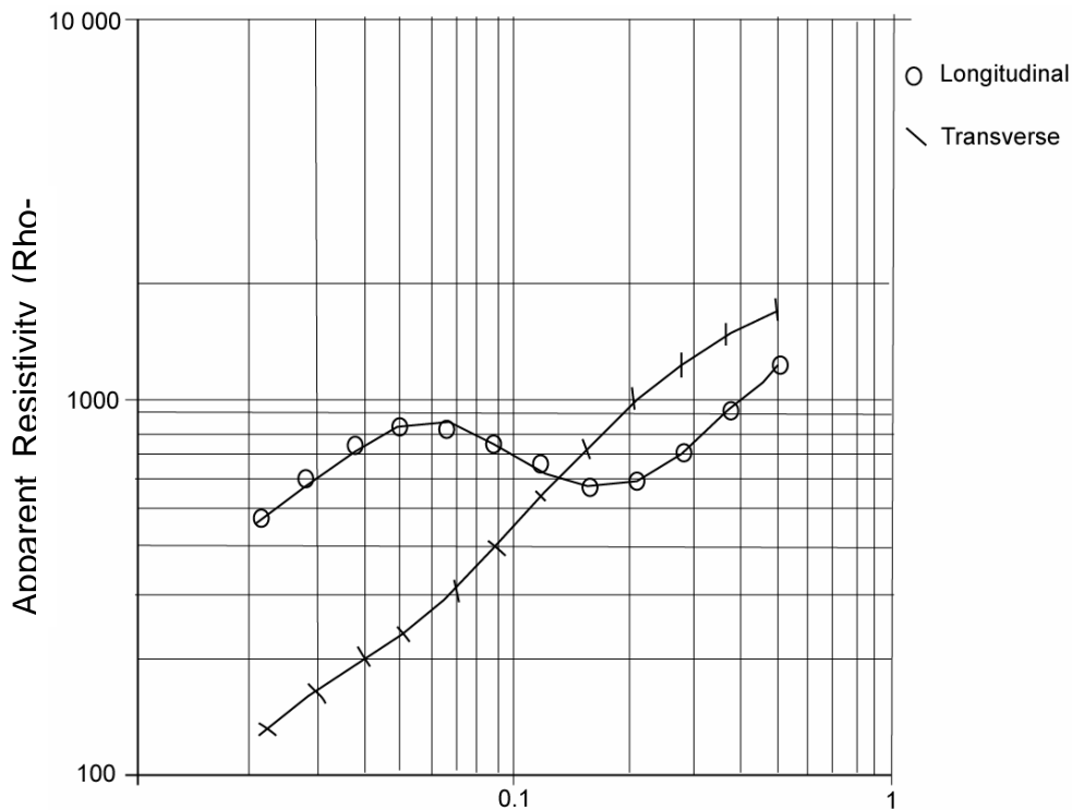
Figure 11. Transverse and longitudinal sounding curves of station A1. Symbols represent the experimental points.
