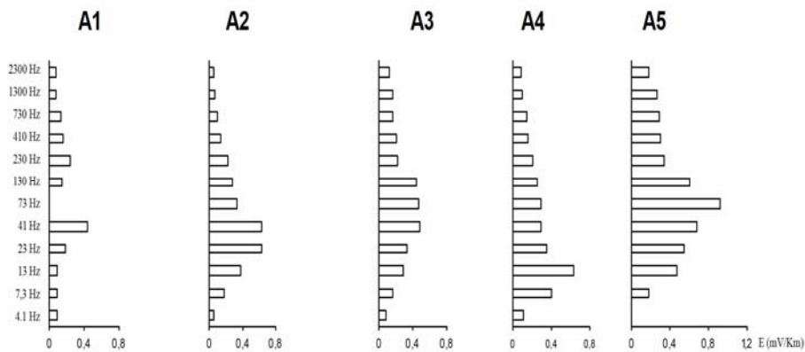
Figure 3a. Propagation of E along profile A telluric line N120°.
