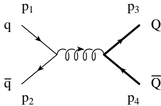
FIG. 1: The lowest order Feynman diagram representing light quark–antiquark annihilation. Normal solid lines represent the light quarks, curly line represents the gluons and the thick solid lines correspond to the heavy quarks.
