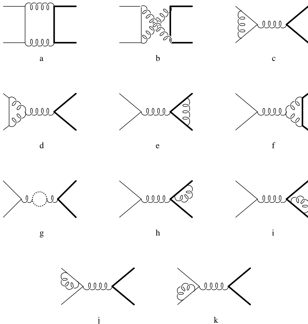
FIG. 2: One-loop Feynman diagrams contributing to the subprocess q\bar{q} \rightarrow Q\bar{Q} . The loop with dotted line in (g) represents gluon, ghost and light and heavy quarks.
