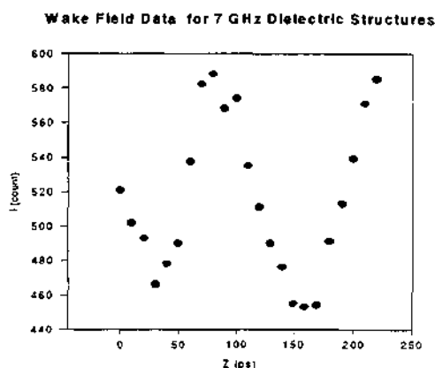
Figure 4. Measured longitudinal wakefield for the 7 GHz dielectric wakefield structure. The peak corresponds to 1.5 MV/m.
