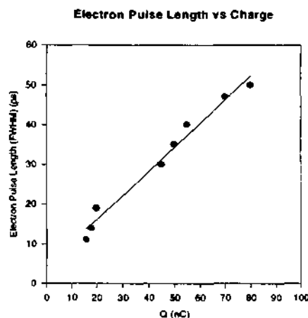
Fig 3 Electron pulse length vs charge
