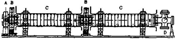
Figure 2. Drive Linac. A: High current photocathode gun. B: Focusing Solenoids (bucking solenoid not shown), C: Linac Cavities, D: Laser and diagnostic port.
