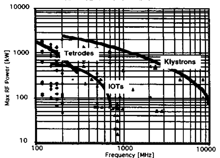
Fig. 3 CW-Rated RF Output Amplifiers Currently Included In ASM RF Power Data Base
