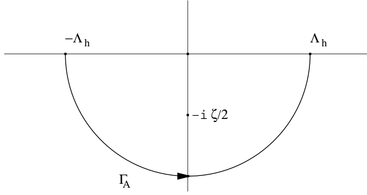
FIG. 3.1 – Contour \Gamma_A
