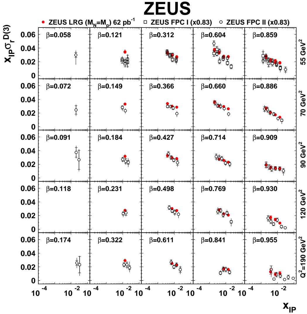
Figure 20: The reduced diffractive cross section multiplied by x_{\mathbb{P}} , x_{\mathbb{P}} \sigma_r^{D(3)} , obtained with the LRG method (dots) as a function of x_{\mathbb{P}} for different values of Q^2 and \beta at high Q^2 . Other details as in caption for Fig. 19.
