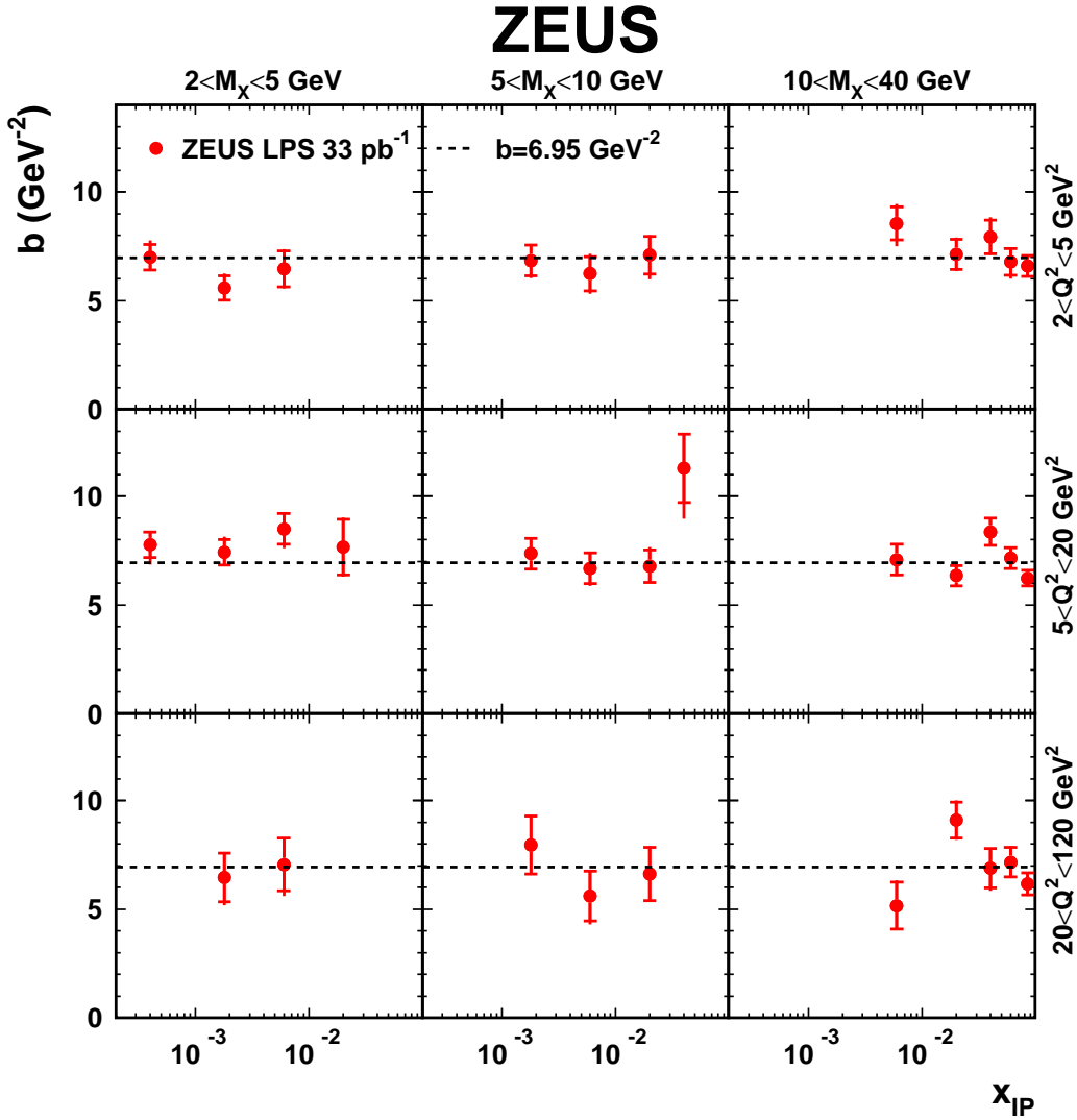
Figure 7: The value of the exponential-slope parameter b of the differential cross-section d\sigma^{ep \rightarrow eXp}/dt \propto e^{-b|t|} as a function of x_{IP} in bins of Q^2 and M_X . The dashed line corresponds to the value of b = 6.95 \text{ GeV}^{-2} , the average t -slope over the measured region. The inner error bars show the statistical uncertainties and the full bars indicate the statistical and the systematic uncertainties added in quadrature.
