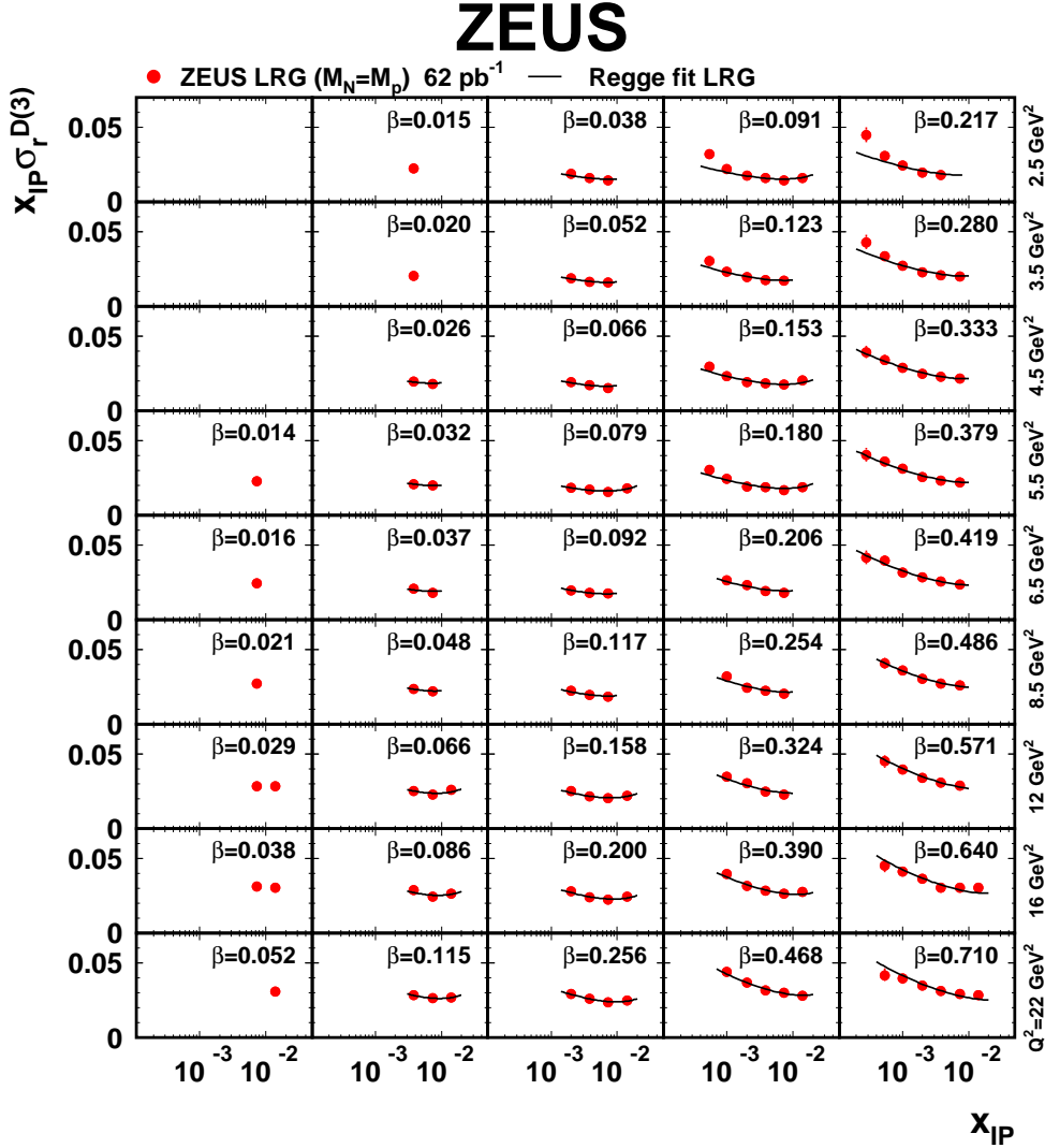
Figure 13: The reduced diffractive cross section multiplied by x_{\mathbb{P}} , x_{\mathbb{P}}^{D(3)} , obtained with the LRG method as a function of x_{\mathbb{P}} for different values of Q^2 and \beta at low Q^2 values. The lines are the result of the Regge fit described in Section 10.5. The inner error bars show the statistical uncertainties and the full bars indicate the statistical and the systematic uncertainties added in quadrature. The data are corrected for the proton-dissociative background to M_N = M_p as described in Section 8.1. The normalisation uncertainty of \pm 5\% is not shown.
