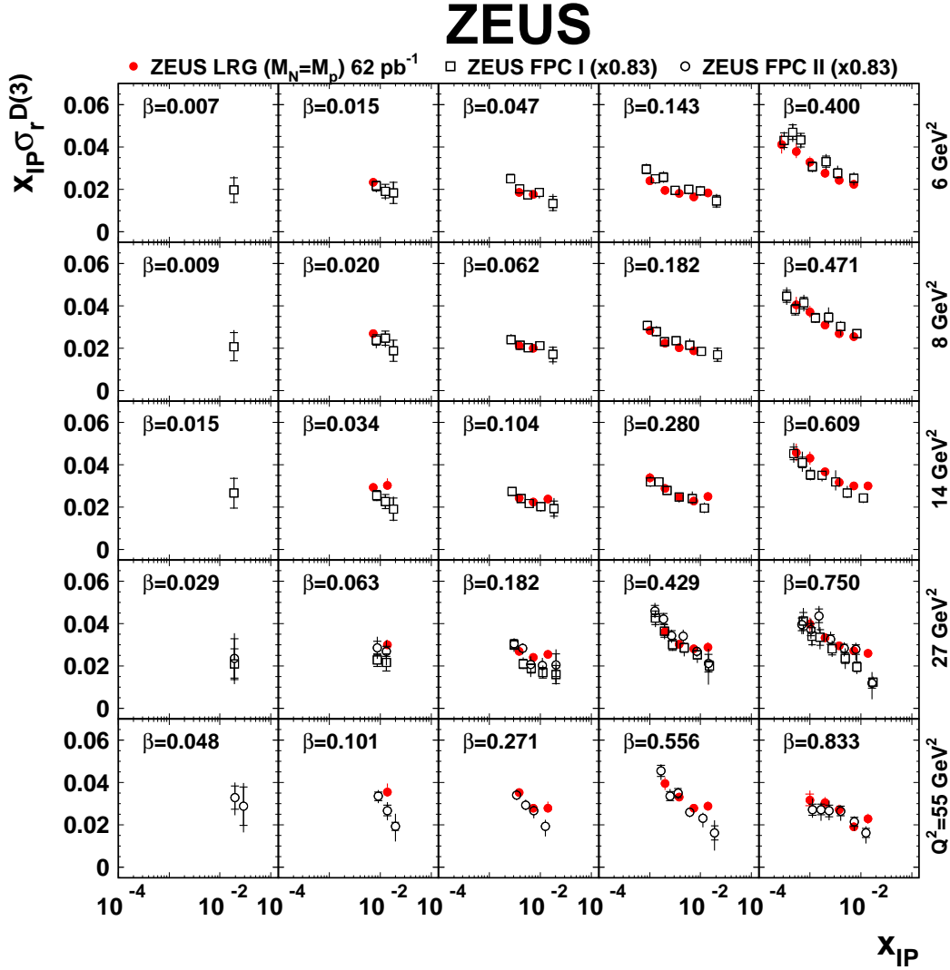
Figure 19: The reduced diffractive cross section multiplied by x_{\mathbb{P}} , x_{\mathbb{P}}\sigma_r^{D(3)} , obtained with the LRG method (dots) as a function of x_{\mathbb{P}} for different values of Q^2 and \beta at low Q^2 , compared with the results obtained with the M_X method, FPC I (open squares) and FPC II (open circles), scaled by the factor 0.83 described in Section 10.4. The inner error bars show the statistical uncertainties and the full bars indicate the statistical and the systematic uncertainties added in quadrature.
