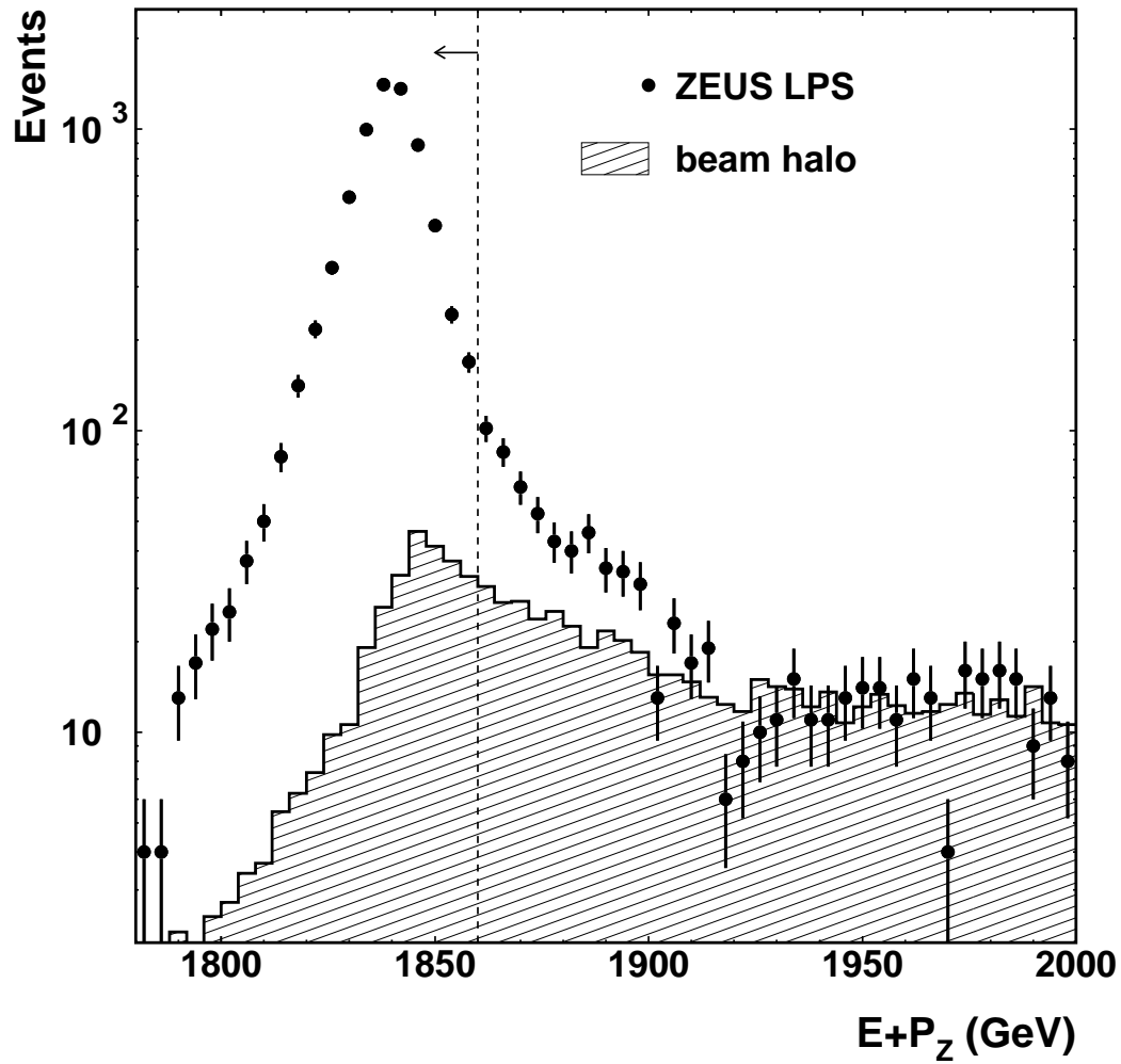
Figure 5: Distribution of E+P_z for the LPS events (dots). The dashed histogram represents the estimate of the beam-halo background normalised for E+P_z > 1925 GeV. The vertical dashed line at E+P_z = 1860 GeV represents the selection cut used in the analysis.
