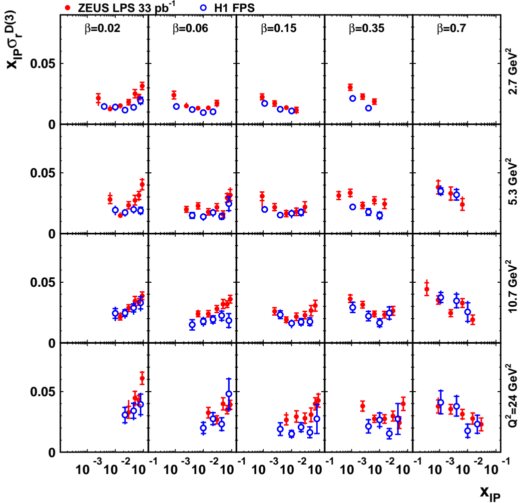
Figure 12: The reduced diffractive cross section multiplied by x_{\mathbb{P}} , x_{\mathbb{P}}\sigma_r^{D(3)} , obtained with the LPS method (dots) as a function of x_{\mathbb{P}} for different values of Q^2 and \beta compared with the results obtained with the H1 Forward Proton Spectrometer (open circles). The inner error bars show the statistical uncertainties and the full bars indicate the statistical and the systematic uncertainties added in quadrature. The normalisation uncertainty of {}_{-7}^{+11}\% of the ZEUS data is not shown, nor is that of the H1 data ( \pm 10\% ).
