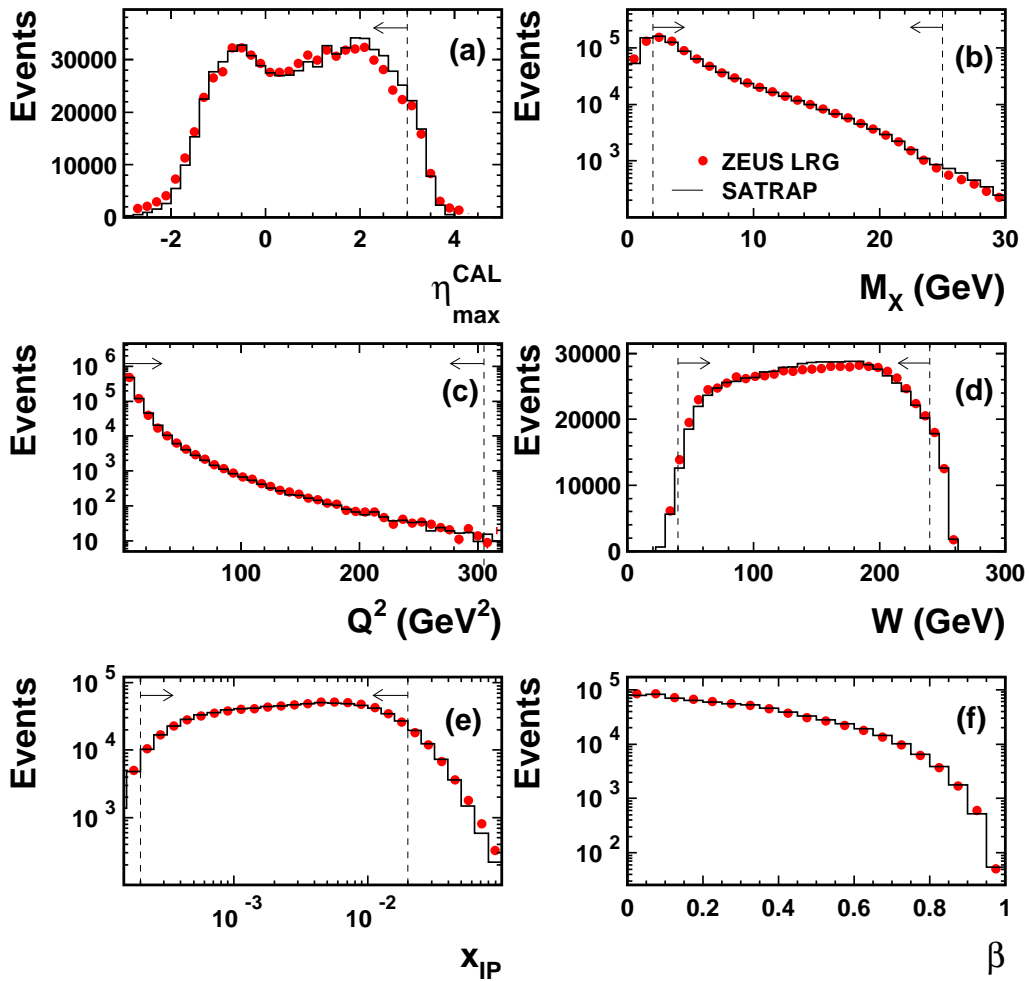
Figure 2: Comparison of the distributions measured (dots) and obtained with the reweighted SATRAP MC (histograms) for (a) \eta_{\text{max}}^{\text{CAL}} , (b) M_X , (c) Q^2 , (d) W , (e) x_{\text{IP}} and (f) \beta in the LRG analysis. For each plot, all analysis cuts have been applied except that on the plotted variable. The vertical lines with arrows indicate the selected region.
