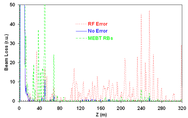
Fig.9 RFQ beam halo loss in the linac in simulation.
