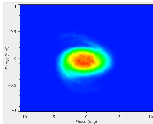
Fig.5 IMPACT predicted profiles at the SCL entrance
