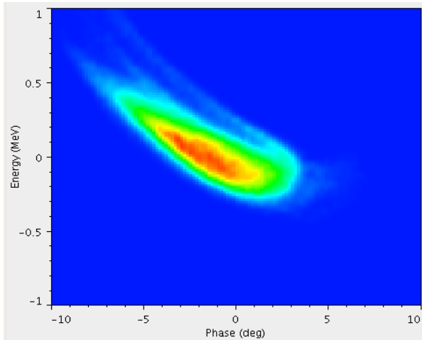
Fig.7 IMPACT model of DTL6 phase shifted by 6°.
