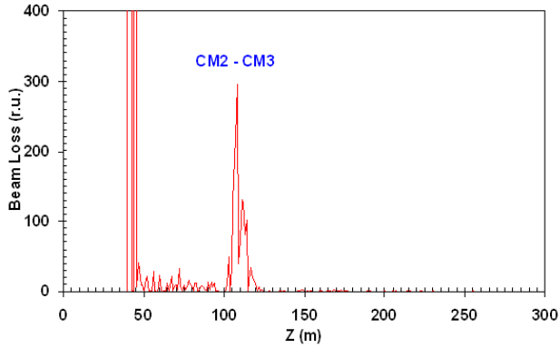
Fig.11 Simulated DTL phase tail loss in the linac.
