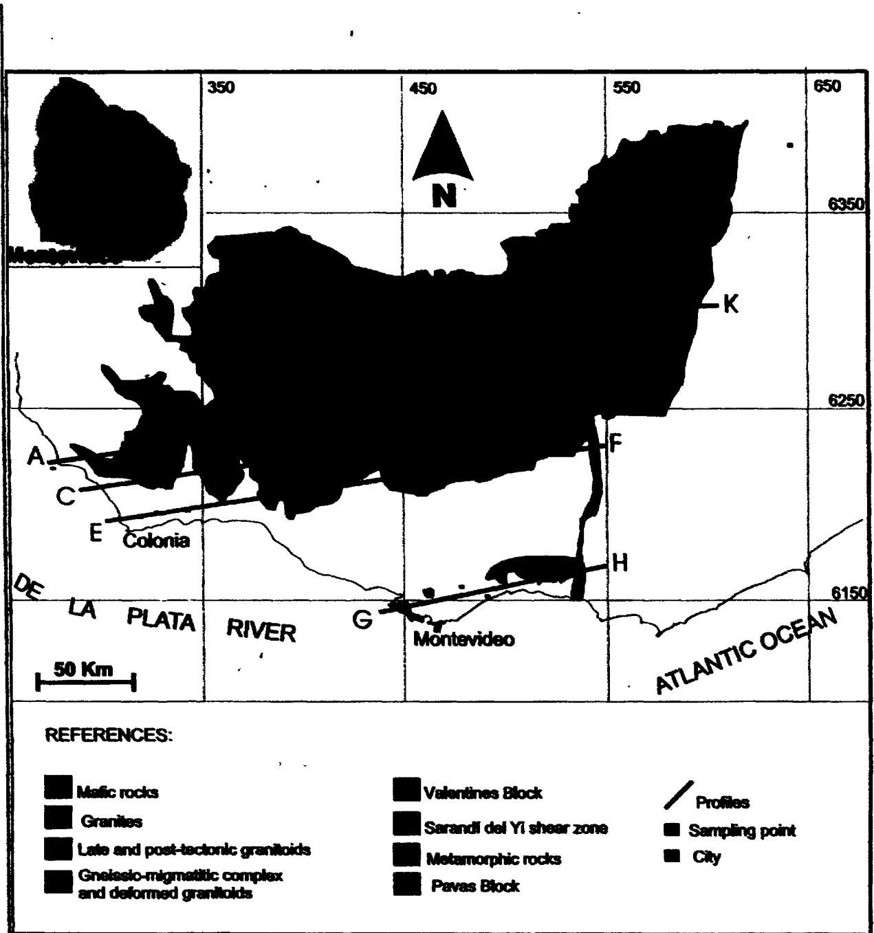
Figure 1. Location map and geologic scheme
