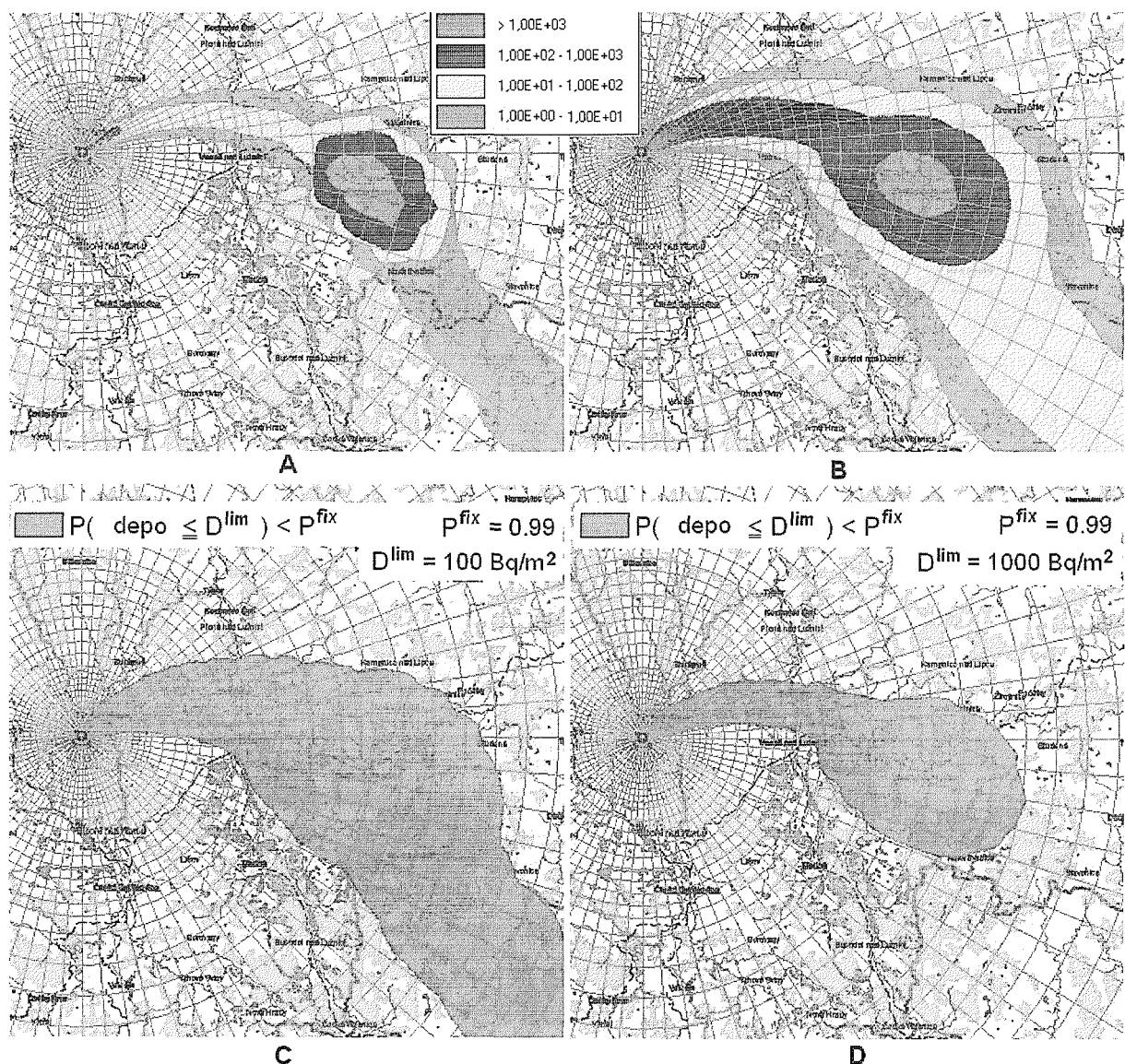
Figure 1. Spatial distribution of ^{137}\text{Cs} activity deposition on terrain [Bq/m 2 ]. Picture of deterministic „best estimate“ (see A); Sample mean (see B); Probability P(\text{depo} \leq D^{\text{lim}}) < P^{\text{fix}} says: deposition limit D^{\text{lim}} will not be exceeded with probability lower then selected number P^{\text{fix}} ; for D^{\text{lim}}=100 \text{ Bq/m}^2 , P^{\text{fix}}=0.99 (see C); for D^{\text{lim}}=1000 \text{ Bq/m}^2 , P^{\text{fix}}=0.99 (see D)
