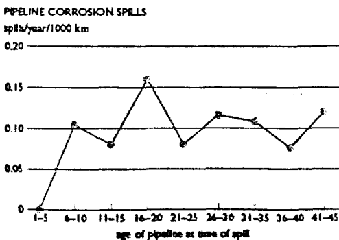
Figure 1 – Rate of Pipeline Failure Due to Corrosion
