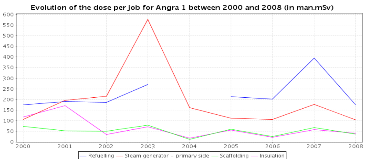
#U-13 Source: ISOE Figure 1 – Evolution of the dose per job for Angra 1
