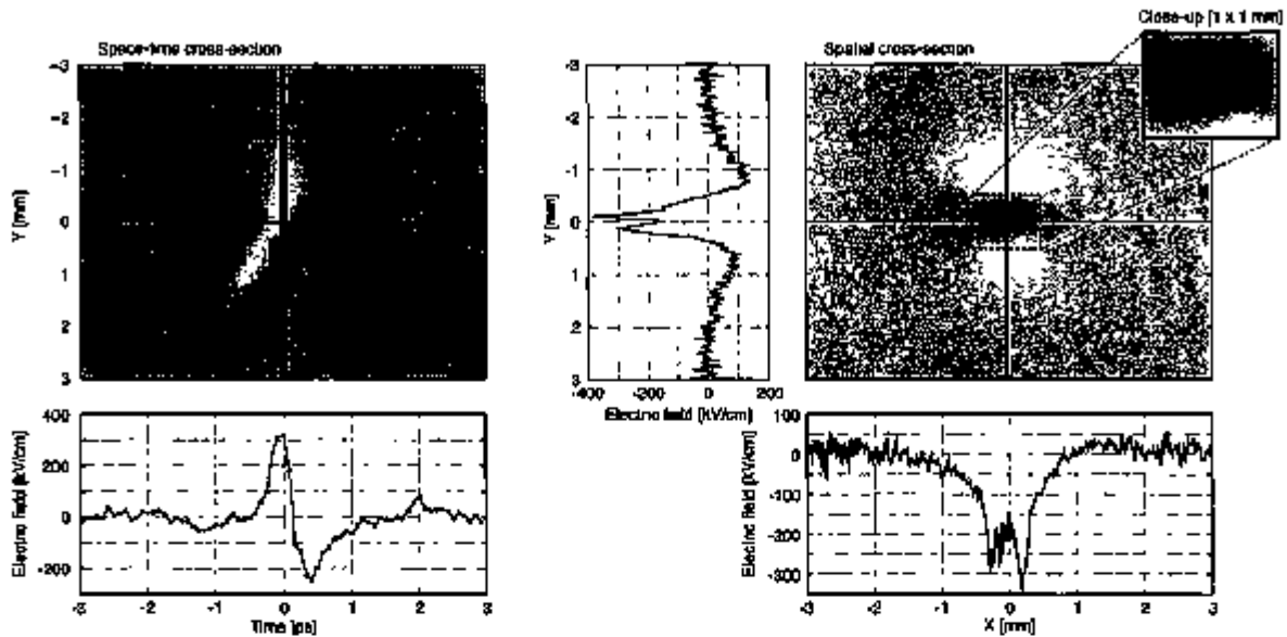
Figure 1: Space-time cross section (left) of the THz pulse electric fields reconstructed from a delay scan using 2D sign-resolved EO sampling. Spatial cross-section (right) showing inversion (close-up).
