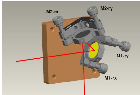
Figure 2. HZB/BESSY-II MBPP design scheme currently used in the NOM.
