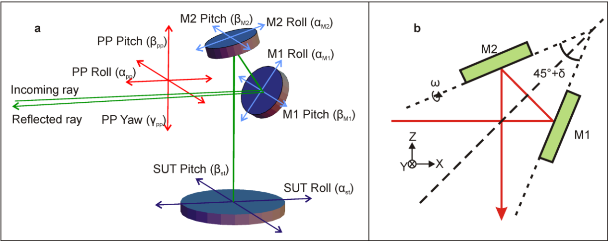
Figure 3. (a) Geometrical representation of the simulated MBPP and surface under test (SUT) system with the relevant coordinate systems. M1 and M2 can be rotated about two axes (M1 and M2 pitch and roll axes), the SUT can be rotated about two axes (SUT pitch and roll axes), and M1 and M2 can be rotated simultaneously about three axes (PP pitch, roll and yaw axes). The deviation of the reflected ray is calculated, simulating an autocollimator measurement. (b) Illustration of the wedge and parallel errors involved in an optical square.
