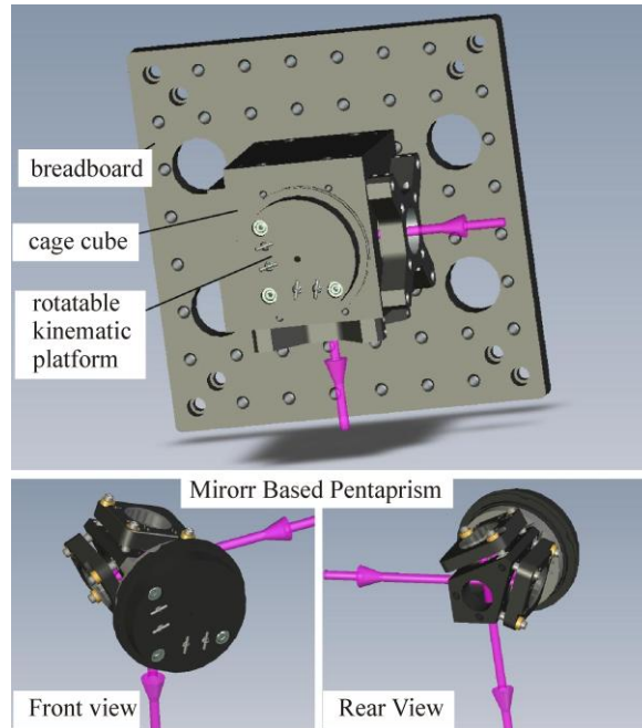
Figure 1. Design of the OML mirror based pentaprism. Most of the parts used are ready to use opto-mechanical components available from Thorlabs, Inc. 12
