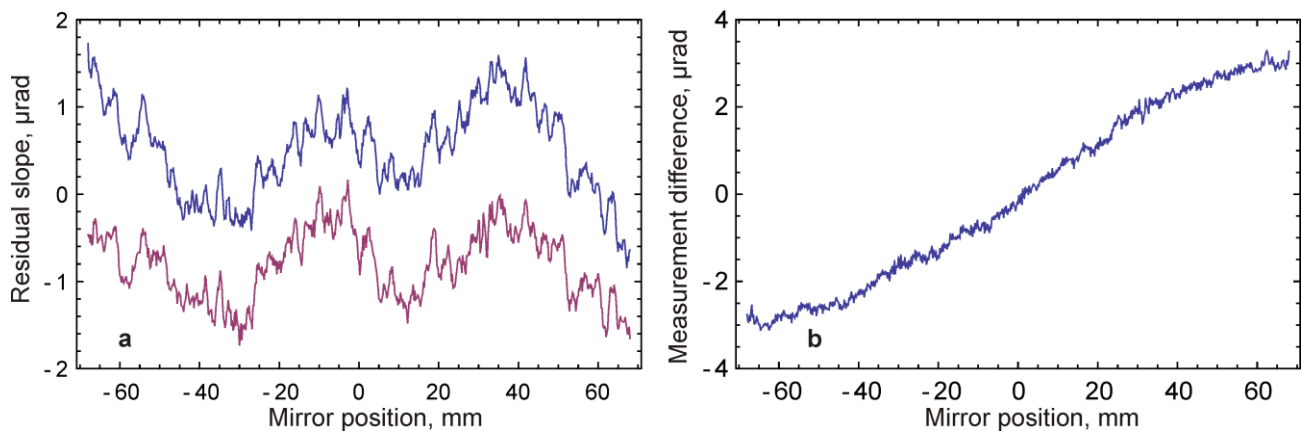
Figure 8. Slope traces of 15 m spherical mirror (a) measured with DLTP equipped with MBPP (bottom line) and pentaprism (top line). Offset is introduced. Difference in the two sets of measurements (b) which represents systematic error associated with bulk pentaprism.
