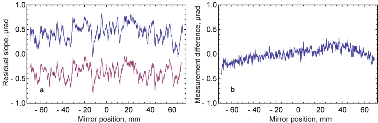
Figure 7. Residual slope traces of flat mirror (a) measured with DLTP equipped with MBPP (bottom line) and pentaprism (top line). The offset is introduced. Difference in the two sets of measurements (b).
