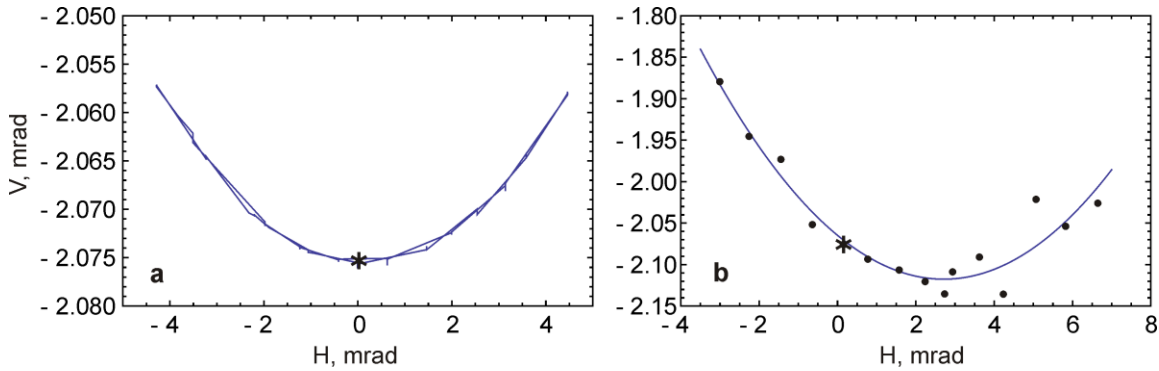
Figure 5. Single roll test with the vertex marked with an asterisk, taken from the series of roll tests performed as M1 is adjusted about its roll axis (a). Quadratic fit of the vertices found from the series of roll tests. The vertex shown in (a) with an asterisk is shown with an asterisk in (b). The parallel error is minimized when H_{roll} = 2.7
