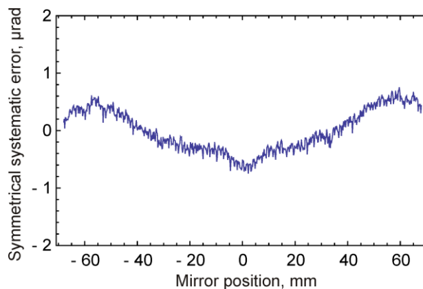
Figure 9. Difference between the forward and reverse measurements of the 15 m optic made with the DLTP equipped with the MBPP. This represents the symmetric error which is removed by averaging the forward and reverse measurements.
