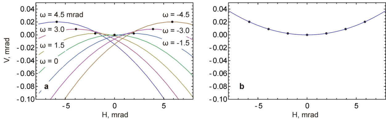
Figure 4. (a) Simulation results of applying a series of roll tests after successively incrementing the parallel error by adjusting the M1 mirror about its roll axis; and (b) a plot of the vertex points with a quadratic fit. The minimum of the quadratic fit in (b) occurs when the parallel error is equal to zero.
