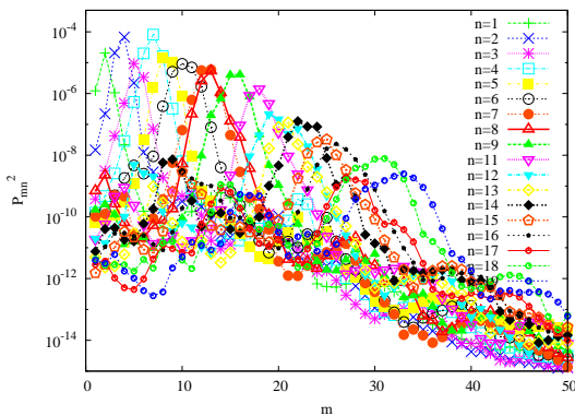
FIG. 4: Fourier amplitudes of the pressure for positive m < 50 and n < 20 . A sum of m and -m is taken.
