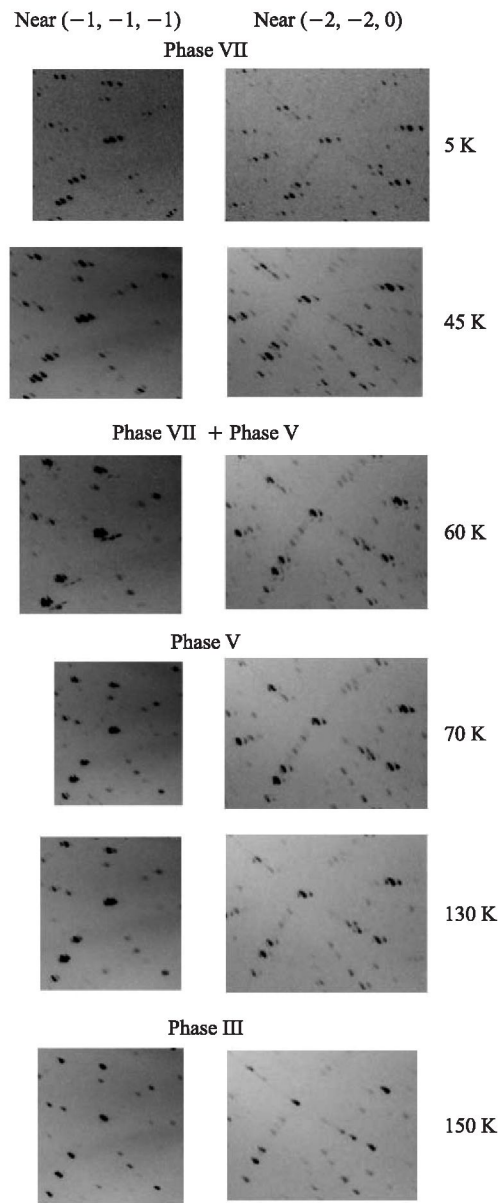
Neutron Laue diffraction patterns from TRAHs ( x = 0.006 ) mixed crystals at different temperatures near (-1, -1, -1) and (-2, -2, 0) Bragg reflections
