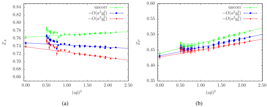
Figure 3: \beta = 1.95 ; dependence of Z_A (left panel) and Z_P (right panel) on (a^2\tilde{p}^2) . Uncorrected and one-loop corrected (with two choices of the gauge coupling, bare and plaquette-boosted) RC estimators are shown.
