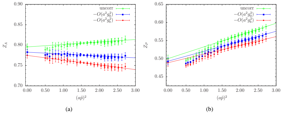
Figure 4: \beta = 2.10 ; dependence of Z_A (left panel) and Z_P (right panel) on (a^2 \tilde{p}^2) . Uncorrected and one-loop corrected (with two choices of the gauge coupling, bare and plaquette-boosted) RC estimators are shown.
