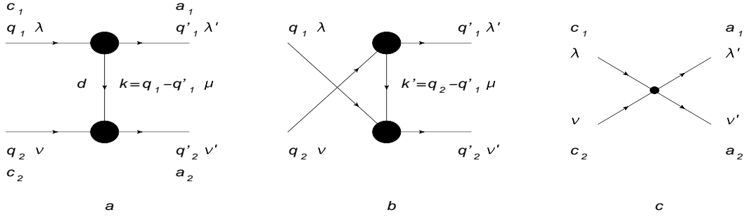
Fig.1: the BFKL kernel.
