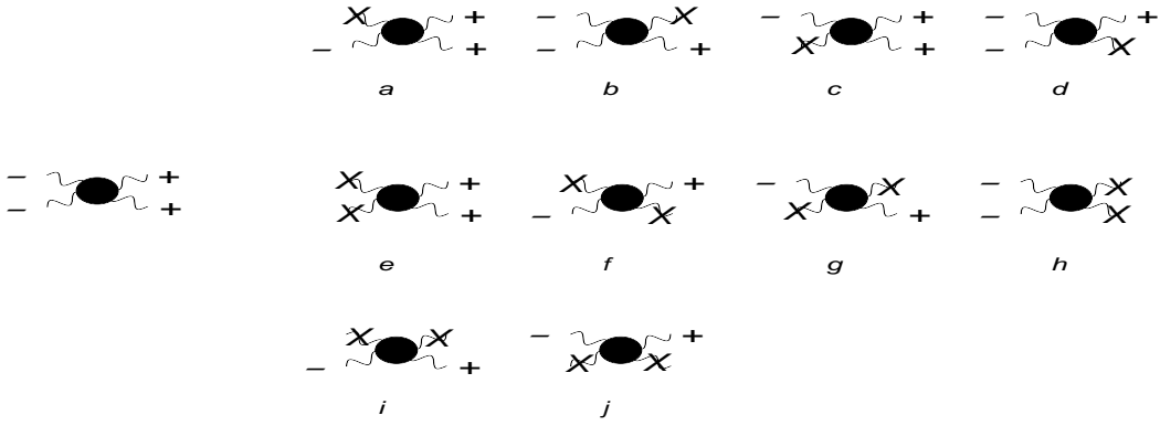
Fig.3: induced vertices in the BFKL kernel.
