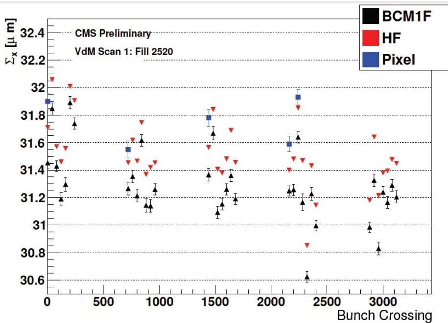
Figure 2. BCM1F luminosity calibration constant compared with other subdetectors. The bunch-by-bunch calibration constant for the x direction \Sigma_x as measured with BCM1F is compared with that measured by other luminosity subdetectors over a full orbit of a van der Meer scan, with agreement of the average values to within 1%.
