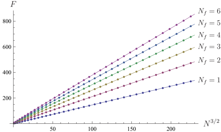
Figure 2. The free energy F = -\log Z for N_f = 1, \dots, 6 as a function of N^{3/2} . The dots represent the exact values computed by our algorithm while the solid lines represent the perturbative part given by the Airy function (3.11).
