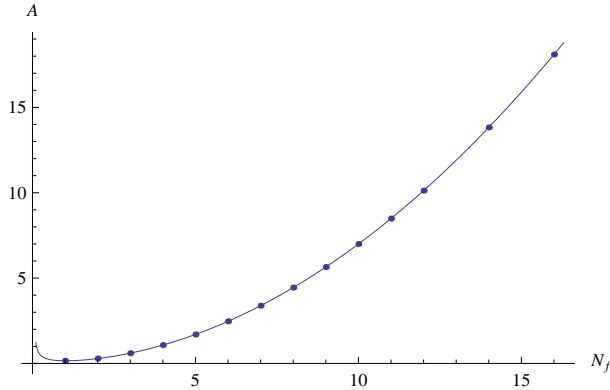
Figure 3. The constant contribution A(N_f) . The numerical estimations (3.18) from exact Z(N_f, N) in the previous section are shown by the dots, and our conjecture (3.12) by the solid line.
