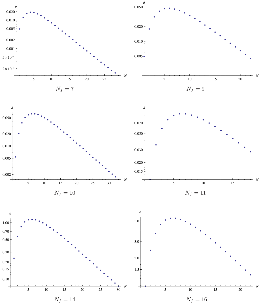
Figure 4. We plot \delta defined in (3.28) for N_f = 7, 9, 10, 11, 14, 16 . Note that the vertical axis is log scale. One can see that \delta is indeed exponentially suppressed as N grows.
