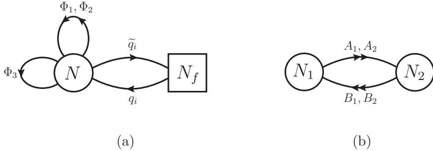
Figure 1. (a) The quiver diagram for the U(N) \mathcal{N} = 4 SYM with an adjoint and N_f fundamental hypermultiplets. We use \mathcal{N} = 2 notation. The adjoint hypermultiplet consists of two adjoint chiral multiplets (\Phi_1, \Phi_2) , and \Phi_3 is the chiral multiplet that forms the \mathcal{N} = 4 vector multiplet together with the \mathcal{N} = 2 vector multiplet. (b) The quiver for the U(N_1)_k \times U(N_2)_{-k} ABJ(M) theory. The partition function of the former with N_f = 1, 2 is related to that of the latter at k = 1, 2 , respectively.
