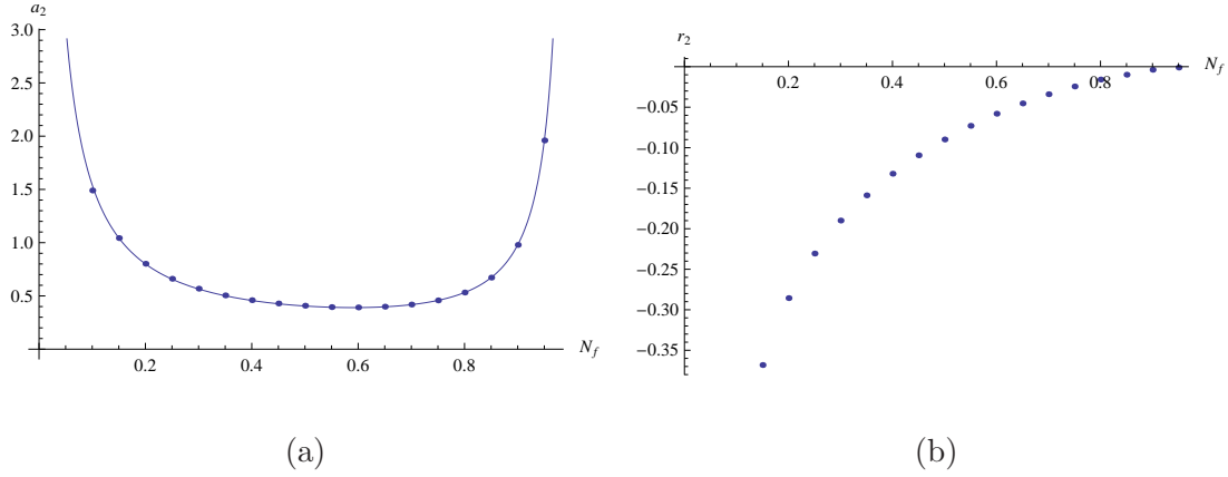
Figure 6. We plot (a) a_2(N_f) and (b) r_2(N_f) = b_2(N_f) - a_2(N_f)/4 against N_f .
