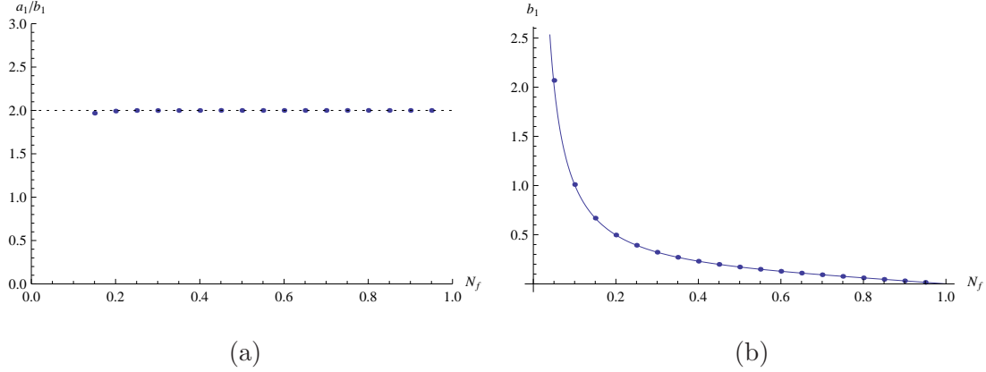
Figure 5. (a) We plot the ratio a_1(N_f)/b_1(N_f) in (4.33) against N_f . These values are estimated by using the TBA equations (2.10) and (2.11). The ratio does not depend on N_f . (b) We compare the analytic conjecture (4.34) with the numerically estimated values from TBA.
