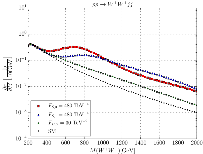
Figure 7: pp \rightarrow W^+W^+jj , unitarized ( QCD contributions neglected).
