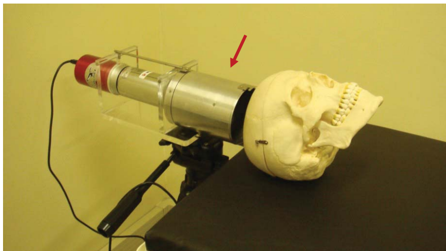
Figure 1. Positioning of the phantom in relation to the detector (indicative arrow).
