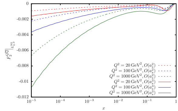
Figure 5: The flavor non-singlet contribution of the Wilson coefficient L_{q,2}^{\text{NS}} to the structure function F_2(x, Q^2) at the 2- and up to the 3-loop order using the NNLO parton distribution functions of Ref. [115] in the on-shell scheme for m_c = 1.59 GeV. Here we do not display the O(a_s^0) terms; from [94].
