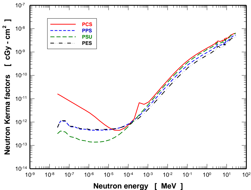
Figure 1.- Neutron kerma factors of PCS, PPS, PSU and PES.
