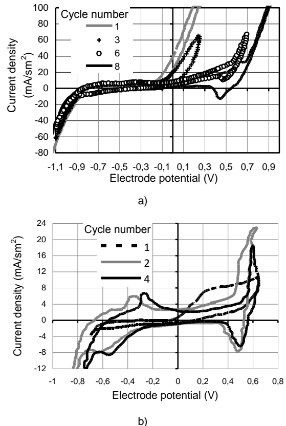
Fig. 1. Cyclic potentiodynamic iE-curves of PVD Mo coatings / Ni coatings with CNM / steel before (a) and after (b) CPF treatment
