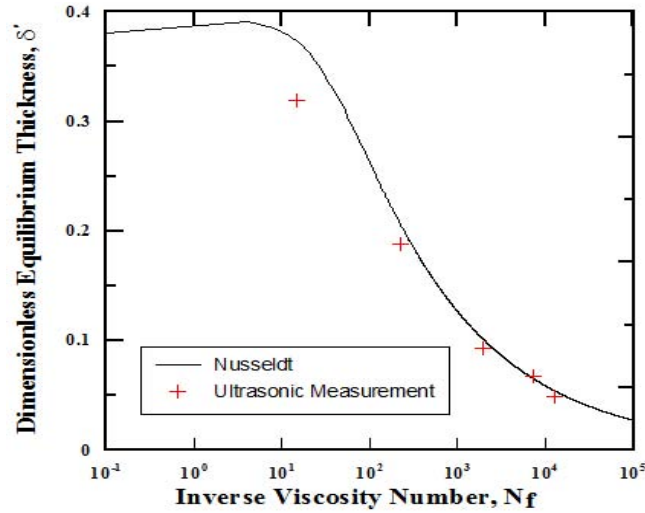
Figure 4: Relationship \delta' vs. N_f for values measured by ultrasound technique and for the Nusseltd [5] correlation.
