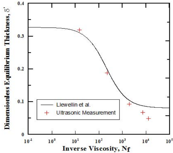
Figure 7: Relationship \delta' vs. N_f for values measured by ultrasound technique and for the Llewellyn et al. [2] correlation.
