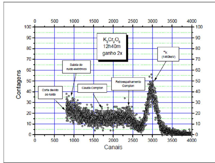
Figure 1: Nuclear Spectrum ^{40}\text{K} , which has an energy 1460 KeV (Silva N. 2005)
