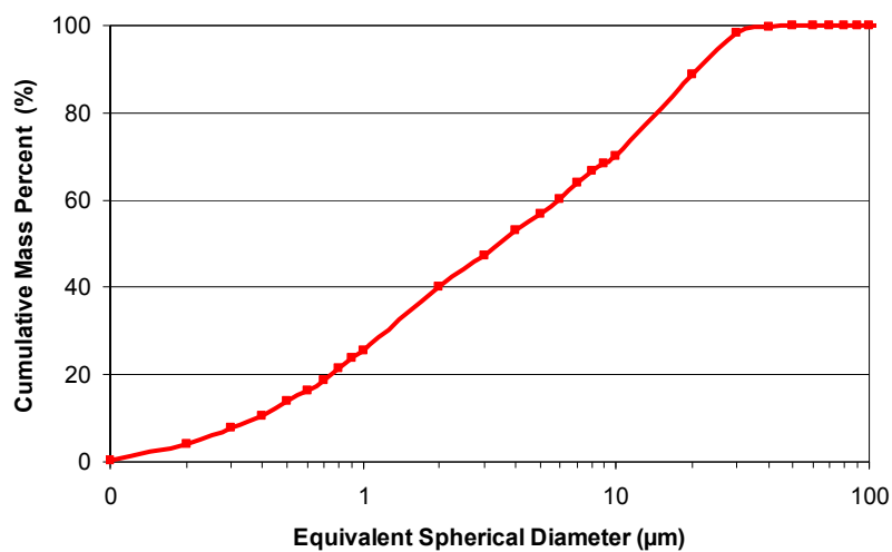
Figure 1. Particle size distribution of the dried red mud.
