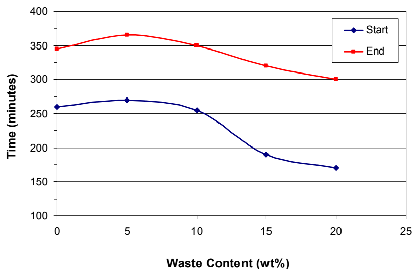
Figure 5. Setting time of Portland cement pastes as a function of red mud content.
