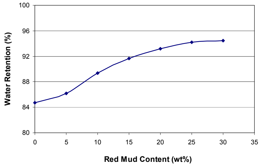
Figure 4. Water Retention of mortars as a function of red mud content.
