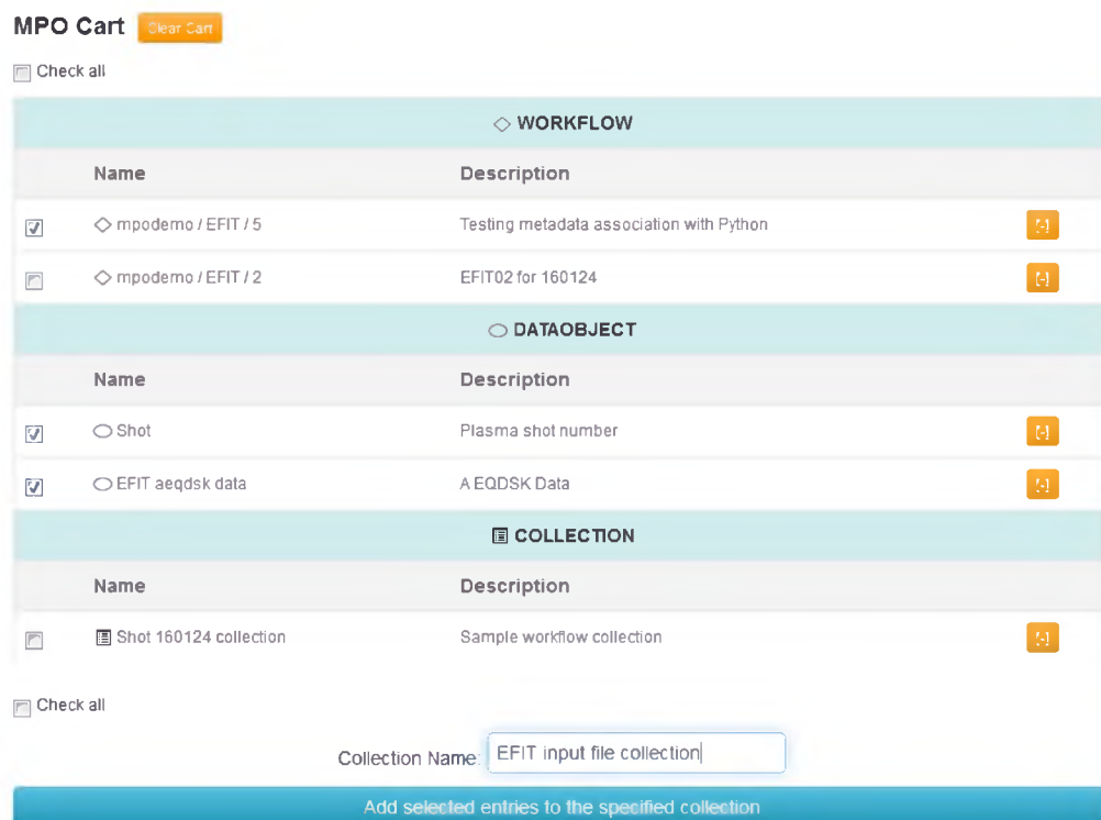
Figure 5. MPO Collection Cart page with Workflow, Data Object and Collection entries. Some entries are selected to be added to the collection, “EFIT input file collection”.
