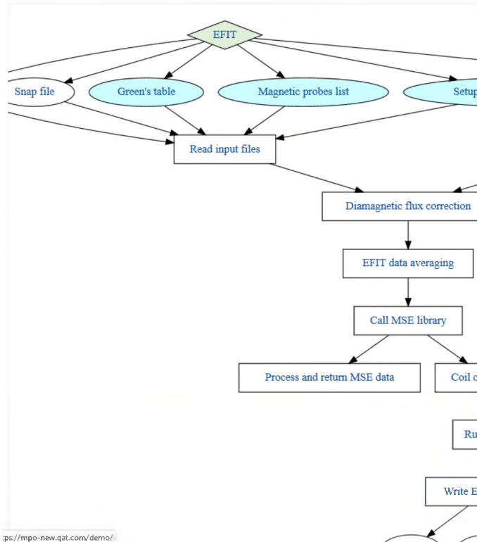
Figure 3. An EFIT workflow displayed on an MPO workflow details page with an interactive DAG and a listing of nodes.
