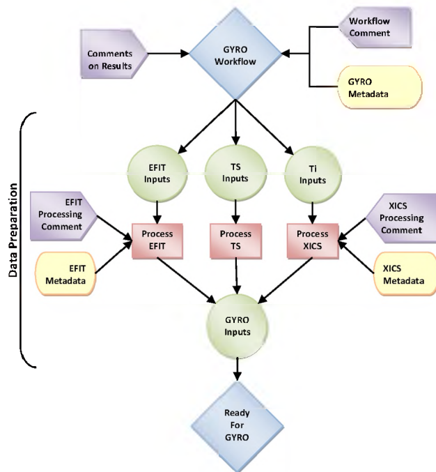
Figure 1. Example data preparation workflow to execute the GYRO code.
