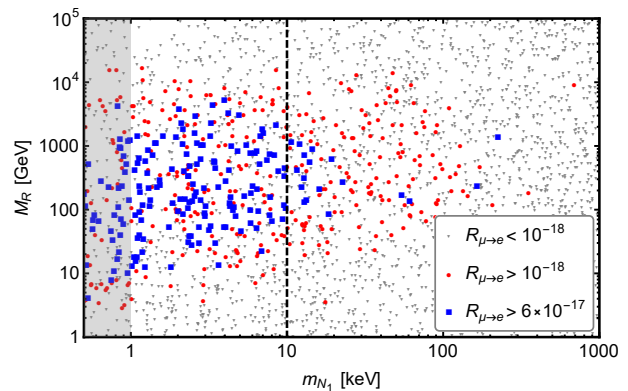
FIG. 2. Results of the numerical scan with \Lambda = 10^{14} GeV, c_h^a = 1 . The shaded region m_{N_1} < 1 keV corresponds to the region excluded the Tremaine-Gunn bound, the dashed line to the structure-formation bound (24).
