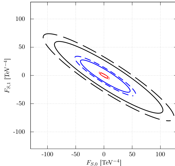
Figure 9: 90 % exclusion sensitivities for polarized (solid) and unpolarized (dashed) particle beams at energies of \sqrt{s} = 1 (black), 1.4 (blue), 3 TeV (red) combined, assuming integrated luminosities of 5 \text{ ab}^{-1} , 1.5 \text{ ab}^{-1} and 2 \text{ ab}^{-1} , respectively.
