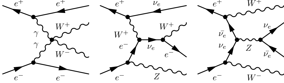
Figure 3: Feynman diagrams contributing to the partially reducible background.
