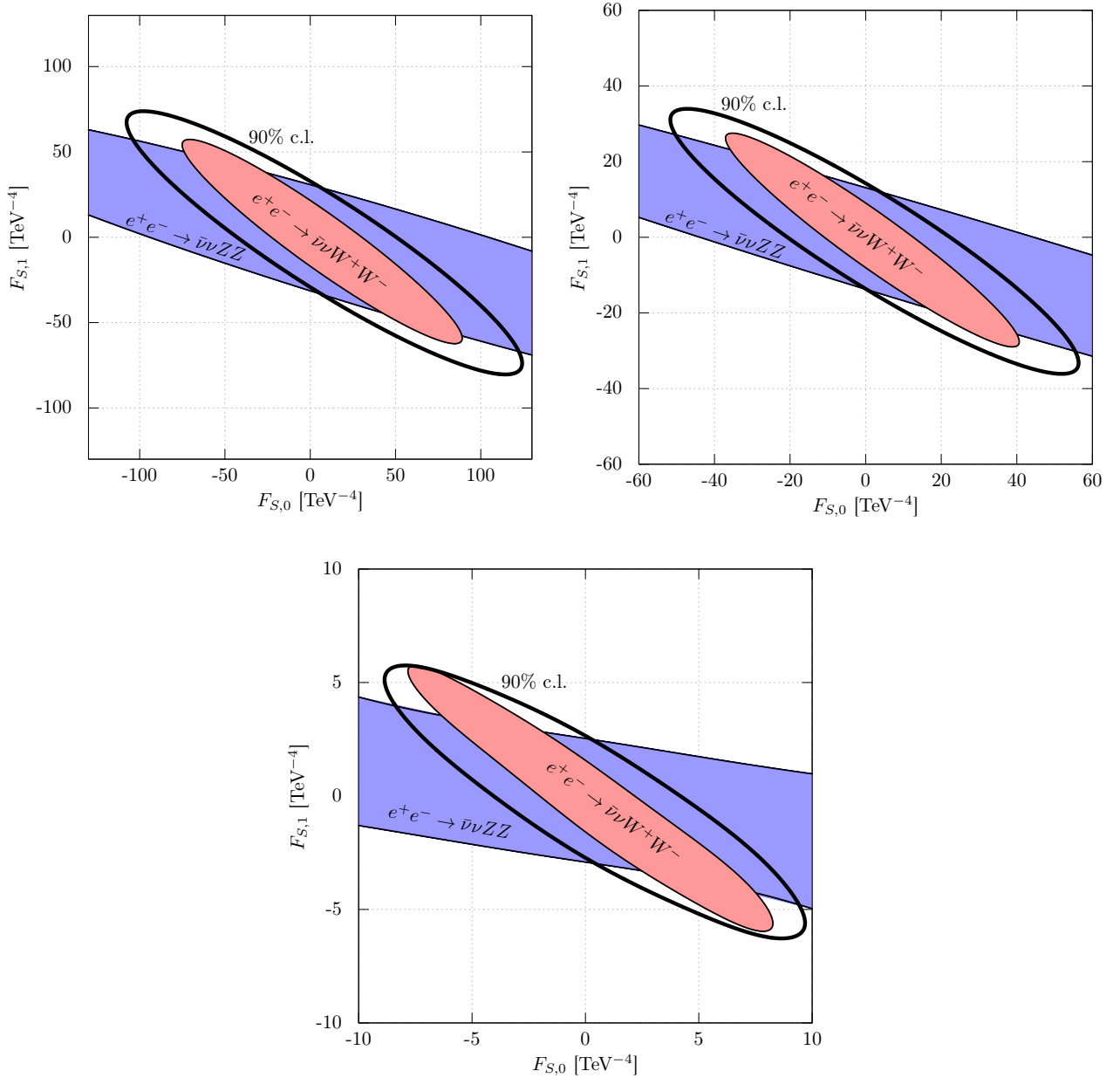
Figure 7: \pm 1\sigma exclusion contours in the F_{S,0}/F_{S,1} plane for the two signal processes e^+e^- \rightarrow \bar{\nu}\nu W^+W^- and e^+e^- \rightarrow \bar{\nu}\nu ZZ including all background processes based on the assumption F_{S,0} = F_{S,1} = 0 . The e^- ( e^+ ) beam is unpolarized at energies of 1.0 TeV (upper left plot), 1.4 TeV (upper right plot) and 3 TeV (lower plot). The corresponding integrated luminosities are 5 ab^{-1} , 1.5 ab^{-1} and 2 ab^{-1} , respectively. All cuts have been applied and detection efficiencies are included. The thick line indicates the 90% exclusion sensitivities obtained by the combination of the two signal channels. All cross sections are unitarized.
