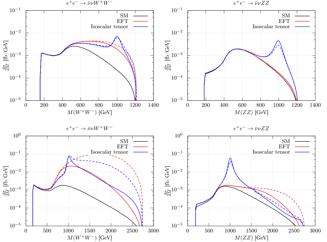
Figure 13: Differential cross sections including an isoscalar tensor resonance ( m_f = 1000 \text{ GeV} , F_f = 17.4 \text{ TeV}^{-1} , \Gamma_f = 100 \text{ GeV} ) depending on the invariant mass of the vector boson pair at center-of-mass energies of \sqrt{s} = 1.4 \text{ TeV} (upper plots) and \sqrt{s} = 3 \text{ TeV} (lower plots). Plots on the left show the process e^+e^- \rightarrow \bar{\nu}\nu W^+W^- , plots on the right e^+e^- \rightarrow \bar{\nu}\nu ZZ . Blue line: isoscalar tensor resonance, red line: matched EFT results ( F_{S,0} = 150.8 \text{ TeV}^{-4} , F_{S,1} = -50.3 \text{ TeV}^{-4} ). Solid line: unitarized results, dashed line: naive results.
