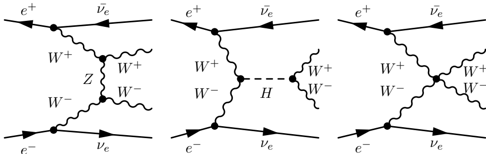
Figure 1: Signal Feynman diagrams contributing to the VBS process.
