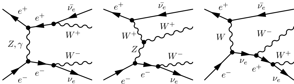
Figure 2: Feynman diagrams contributing to the irreducible background.
