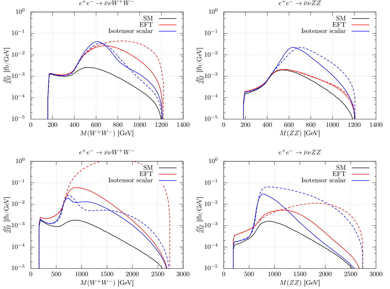
Figure 14: Differential cross sections including a low lying isotensor scalar resonance ( m_\phi = 650 GeV, F_\phi = 19.5 TeV ^{-1} , \Gamma_\phi = 260 GeV) depending on the invariant mass of the vector boson pair at center-of-mass energies of \sqrt{s} = 1.4 TeV (upper plots) and \sqrt{s} = 3 TeV (lower plots). Plots on the left show the process e^+e^- \rightarrow \bar{\nu}\nu W^+W^- , plots on the right e^+e^- \rightarrow \bar{\nu}\nu ZZ . Blue line: isotensor scalar resonance, red line: matched EFT results ( F_{S,0} = 450.5 TeV ^{-4} , F_{S,1} = -112.6 TeV ^{-4} ). Solid line: unitarized results, dashed line: naive results.
