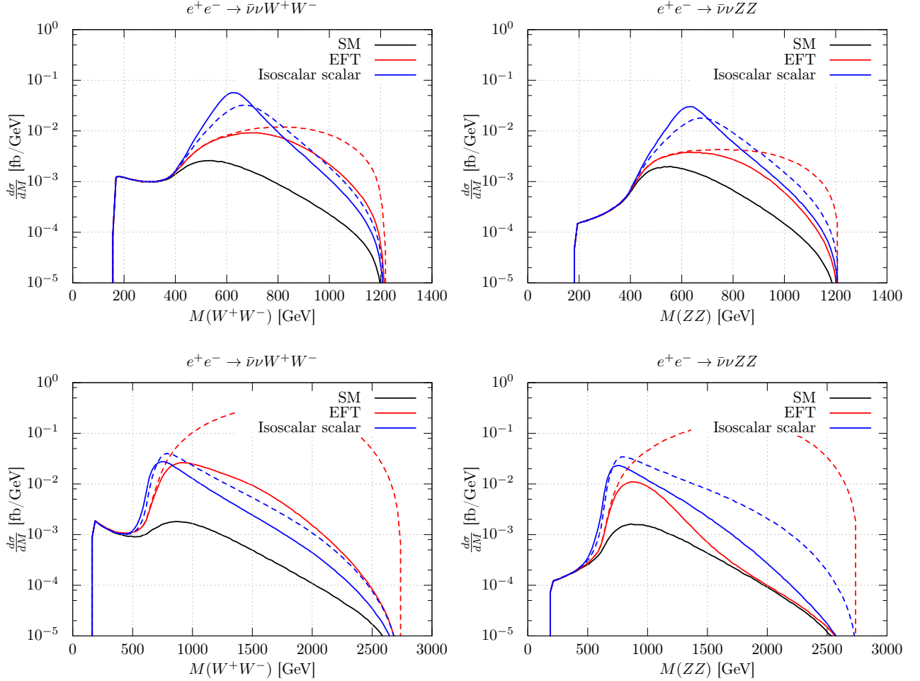
Figure 12: Differential cross sections including a low lying isoscalar scalar resonance ( m_\sigma = 650 GeV, F_\sigma = 9.8 TeV ^{-1} , \Gamma_\sigma = 260 GeV) depending on the invariant mass of the vector boson pair at center-of-mass energies of \sqrt{s} = 1.4 TeV (upper plots) and \sqrt{s} = 3 TeV (lower plots). Plots on the left show the process e^+e^- \rightarrow \bar{\nu}\nu W^+W^- , plots on the right e^+e^- \rightarrow \bar{\nu}\nu ZZ . Blue line: isoscalar scalar resonance, red line: matched EFT results ( F_{S,0} = 0 , F_{S,1} = 112.6 TeV ^{-4} ). Solid line: unitarized results, dashed line: naive results.
