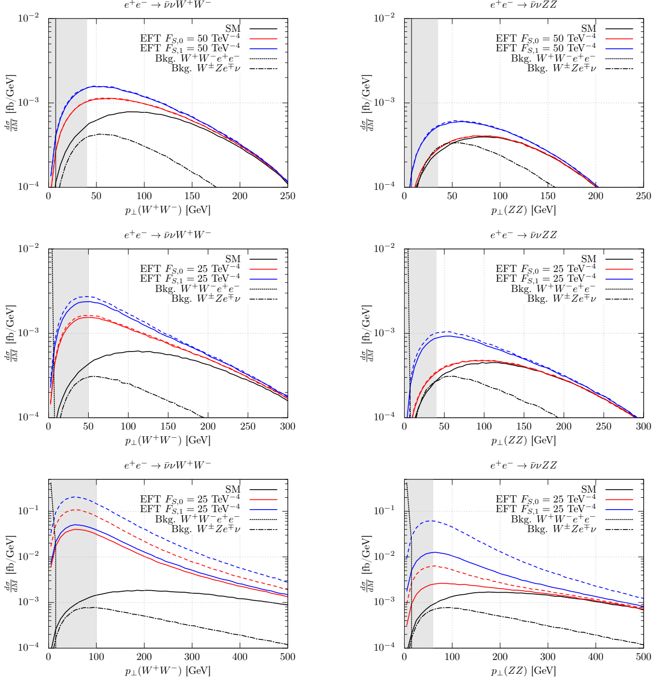
Figure 4: Differential cross sections depending on the transverse momentum of the W (left plots) and the Z boson pair (right plots) at center-of-mass energies of 1 TeV (upper plots), 1.4 TeV (middle plots) and 3 TeV (lower plots). The solid lines show the signal process \bar{\nu}\nu W^+W^- ( ZZ ) with SM values F_{S,0} = F_{S,1} = 0 . The red/blue lines indicate the signal process with non SM value F_{S,0,1} = 25/50 \text{ TeV}^{-4} (dashed lines: naive EFT results, solid lines: unitarized results). In addition, the two SM background processes W^+W^-e^+e^- and W^{\pm}Ze^{\mp}\nu (with 13.6% misidentification probability) are also plotted. The shaded area is removed by the cut on the W ( Z ) boson system. All other cuts have been applied as described. No detection efficiencies are included.
