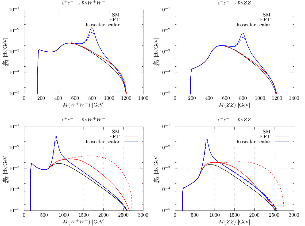
Figure 11: Differential cross sections including a weakly coupled isoscalar scalar resonance ( m_\sigma = 800 GeV, F_\sigma = 4.0 TeV ^{-1} , \Gamma_\sigma = 80 GeV) depending on the invariant mass of the vector boson pair at center-of-mass energies of \sqrt{s} = 1.4 TeV (upper plots) and \sqrt{s} = 3 TeV (lower plots). Plots on the left show the process e^+e^- \rightarrow \bar{\nu}\nu W^+W^- , plots on the right e^+e^- \rightarrow \bar{\nu}\nu ZZ . Blue line: isoscalar scalar resonance, red line: matched EFT results ( F_{S,0} = 0 , F_{S,1} = 12.3 TeV ^{-4} ). Solid line: unitarized results, dashed line: naive results.
