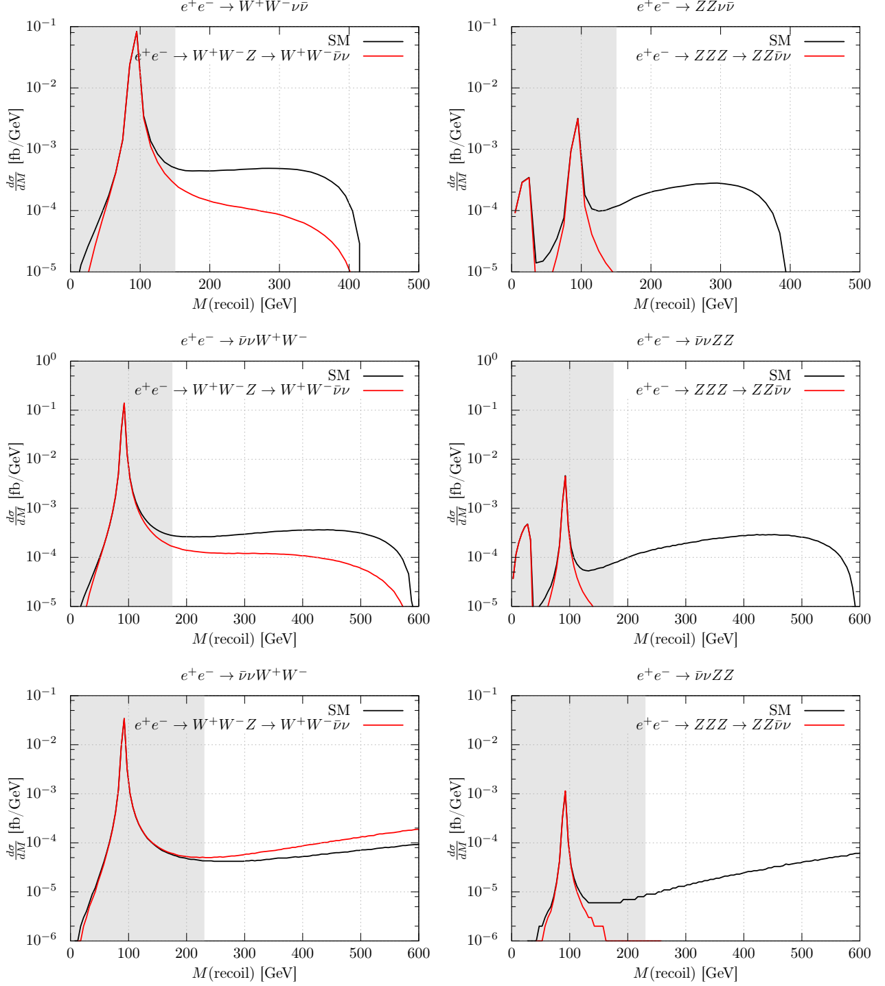
Figure 6: Differential cross sections depending on the recoil mass of the W (left plots) and the Z boson pair (right plots) at center-of-mass energies of 1 TeV (upper plots), 1.4 TeV (middle plots) and 3 TeV (lower plots). The solid lines show the signal process \bar{\nu}\nu W^+W^- (ZZ) . The red lines show the background process e^+e^- \rightarrow W^+W^-(ZZ)Z \rightarrow W^+W^-(ZZ)\nu\bar{\nu} , where the two neutrinos are generated through a decaying Z boson. The shaded area is removed by the cut on the neutrino system. All other cuts have been applied as described above. No detection efficiencies are included.
