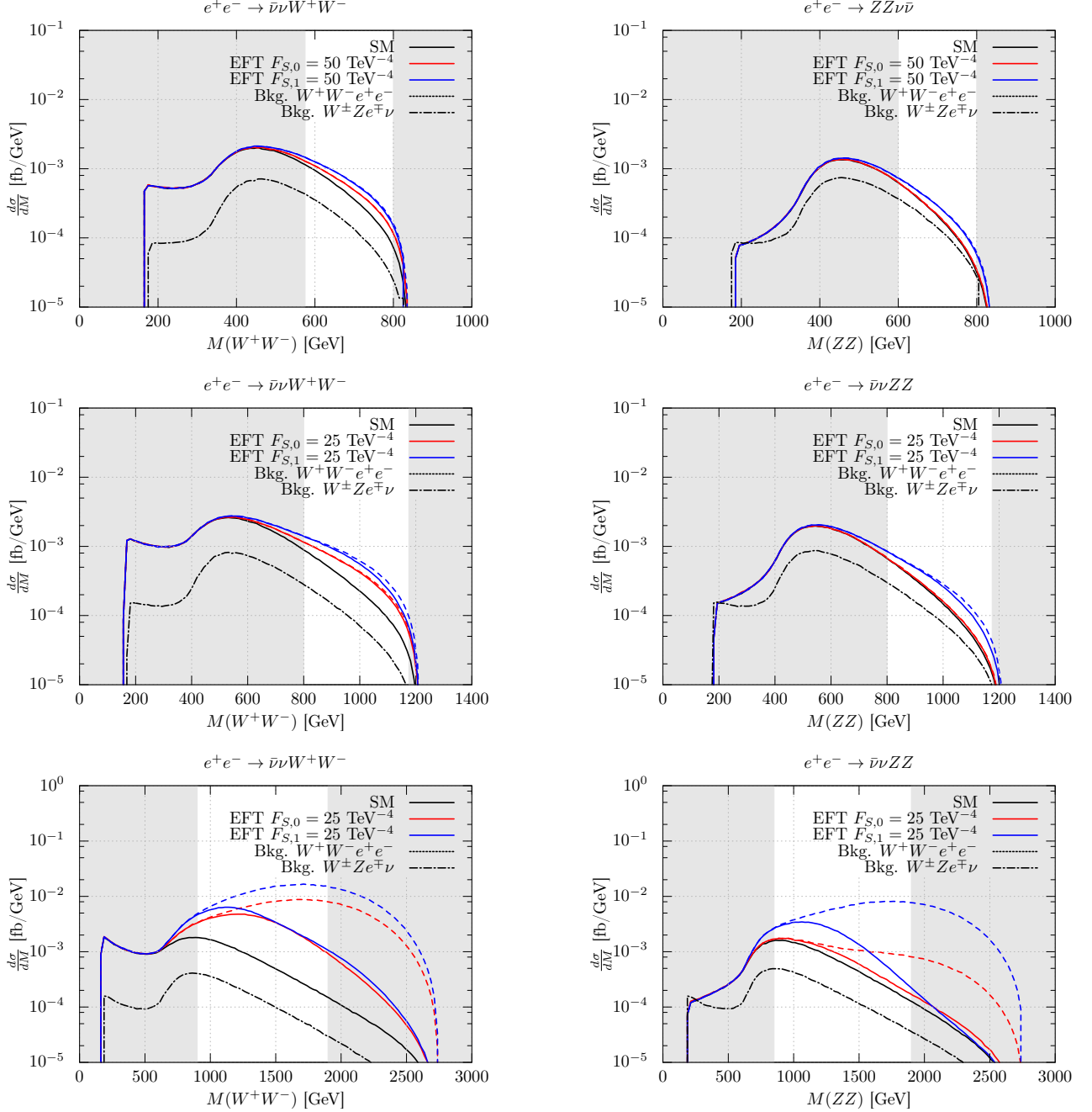
Figure 5: Differential cross sections depending on the invariant mass of the W (left plots) and the Z boson pair (right plots) at center-of-mass energies of 1 TeV (upper plots), 1.4 TeV (middle plots) and 3 TeV (lower plots). The solid lines show the signal process \bar{\nu}\nu W^+W^- ( ZZ ) with SM values F_{S,0} = F_{S,1} = 0 . The red/blue lines indicate the signal process with non SM value F_{S,0,1} = 25/50 \text{ TeV}^{-4} (dashed lines: naive EFT results, solid lines: unitarized results). In addition, the two SM background processes W^+W^-e^+e^- and W^\pm Ze^\mp\nu (with 13.6% misidentification probability) are also plotted. The shaded area is removed by the cut on the W(Z) boson system. All other cuts have been applied as described. No detection efficiencies are included.
