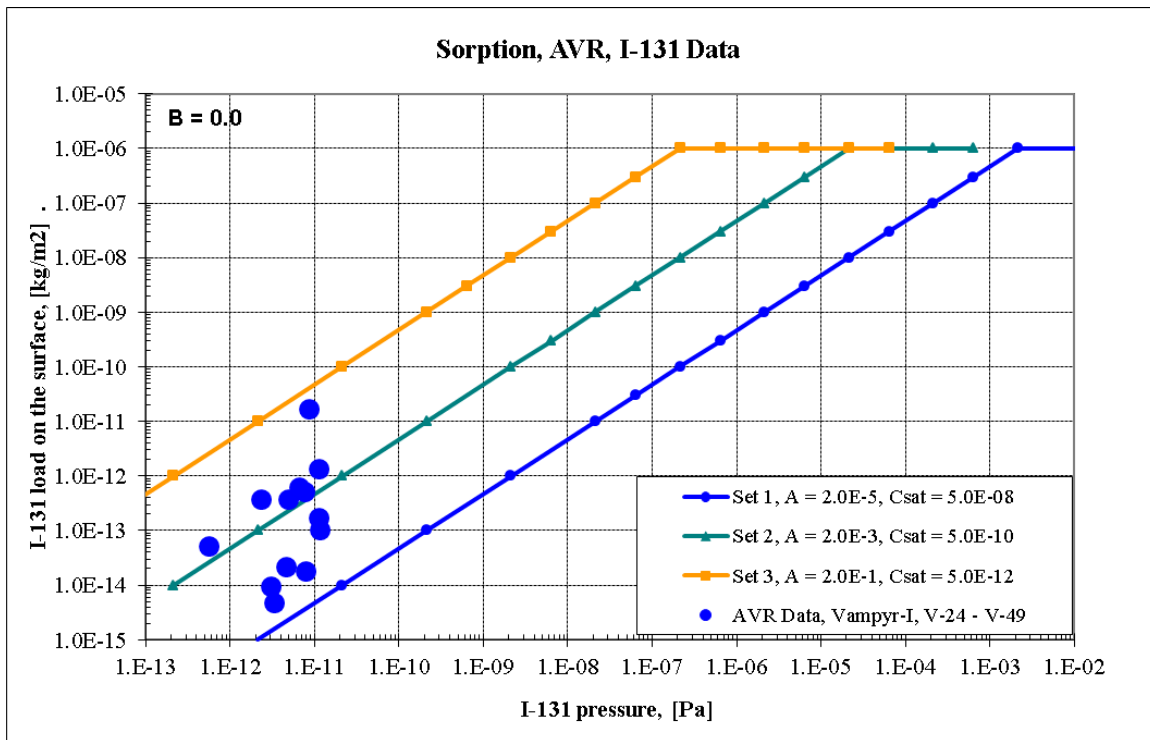
Figure 3-2 I-131 - AVR data and Langmuir isotherms, B_S = 0.0
