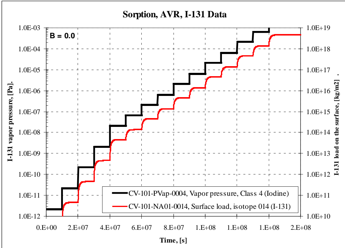
Figure 3-1 I-131 - AVR data and Langmuir isotherms, B_S = 0.0
