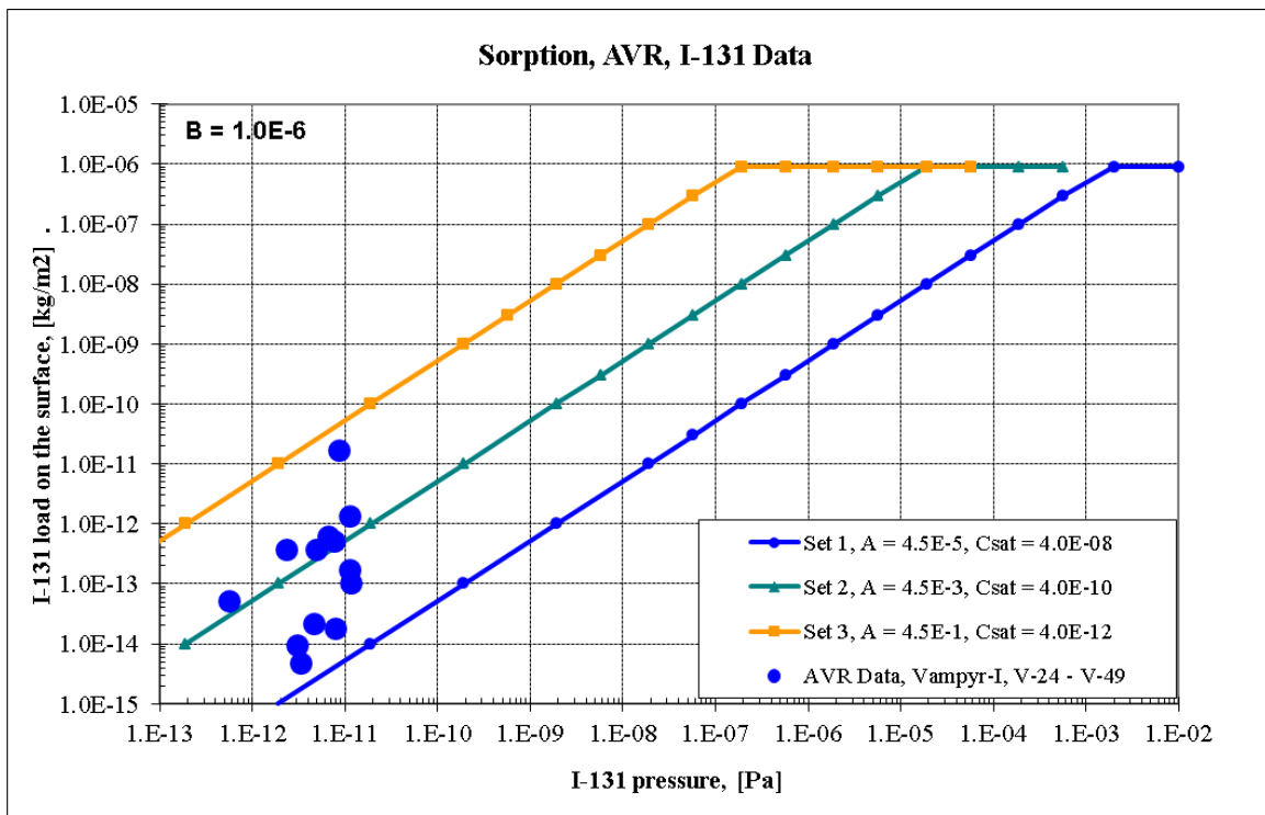
Figure 3-4 I-131 - AVR data and Langmuir isotherms
