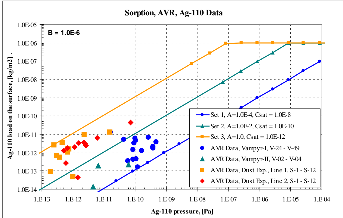
Figure 3-5 Ag-110m - AVR data and Langmuir isotherms
