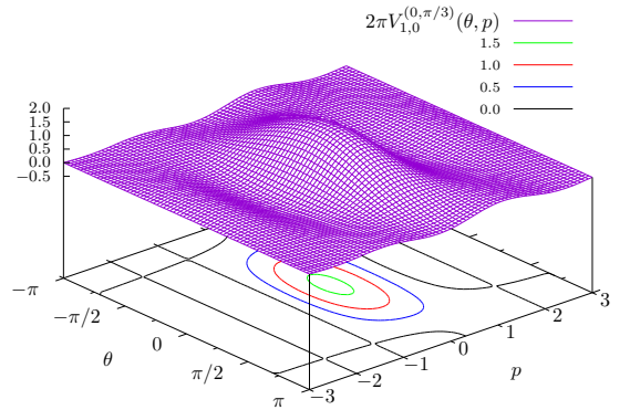
FIG. 2. A-OAM Wigner function 2\pi V_{1,0}^{(\alpha=0, \beta=\pi/3)}(\theta, p) = \frac{1}{4}[\operatorname{sinc} \pi(p - 1) + 3 \operatorname{sinc} \pi p] + \frac{\sqrt{3}}{2} \cos \theta \operatorname{sinc} \pi(p - 1/2) for the qubit (e_{+1} + e_0)/\sqrt{2} .
