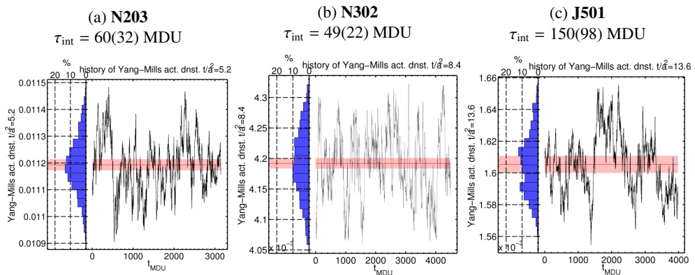
Figure 4: History of the YM action density at flow time t_0 along the MD trajectory. The three panes show results for a \approx 0.064 fm (a), a \approx 0.050 fm (b), and a \approx 0.039 fm (c).
