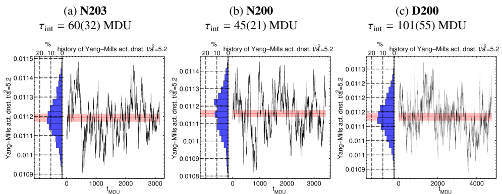
Figure 5: History of the YM action density at flow time t_0 along the MD trajectory. The three panes show results at fixed lattice spacing a \approx 0.064 fm for m_\pi \approx 340 MeV (a), m_\pi \approx 280 MeV (b), and m_\pi \approx 200 MeV (c).
