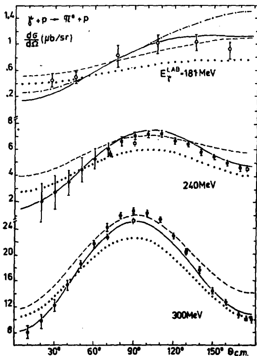
Fig. 2. The same as in fig. 1 for angular distributions. Data are from ref. [13] ( \circ ), [14] ( \square ) and [15] ( \triangle ).
