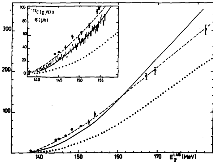
Fig. 3. The \pi^0 -coherent photoproduction cross-section on carbon. The meaning of the curves is the same as in fig. 1. experimental points from ref.[9], \square - preliminary data from the Mainz-Giessen collaboration.
