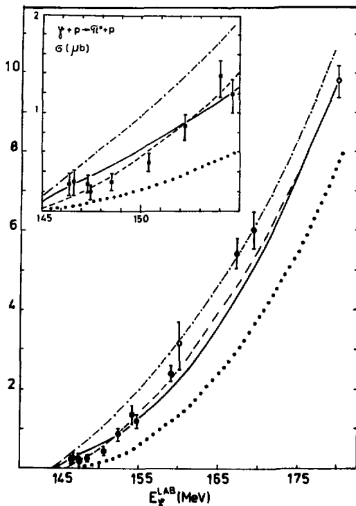
Fig. 1. The \pi^0 - photoproduction cross-section on the proton calculated using BL - amplitude with R_w = 0 (dash-dotted line), R_w = -0.28 (dashed line) and using BDW - amplitude with G_w^V = 0 , R_w = 0 (dotted line) and G_w^V = 10 , R_w = 0.43 (full line). Data are from ref. [1] ( \phi ) and [12] ( \phi ).
