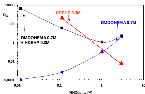
Fig 2. Europium extraction ( D_{Eu} ) v.s. aqueous nitric acid concentration. Organic phases: red 0.3M HDEHP in dodecane, blue 0.7 M DMDOHEMA in dodecane, black 0.7 M DMDOHEMA + 0.3 M HDEHP in n-dodecane.
