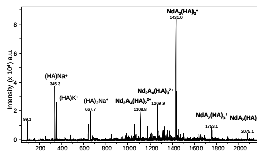
Fig. 5. Positive ESI-MS of 0.1M HDEHP in dodecane after contact with 1M Nd(NO_3)_3 in 0.1 M nitric acid. AH represents HDEHP.
