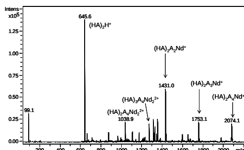
Fig. 4. Positive ESI-MS of 0.3M HDEHP in dodecane after contact with 0.1 M Nd(NO_3)_3 in 0.1 M nitric acid. AH represents HDEHP
